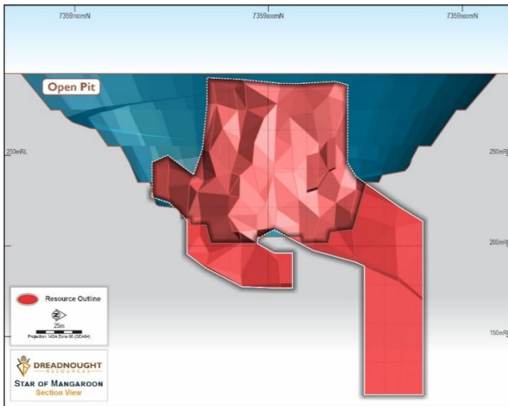
Figure 5 (above): Long section (looking west) of the Star of Mangaroon open pit design and Resource
