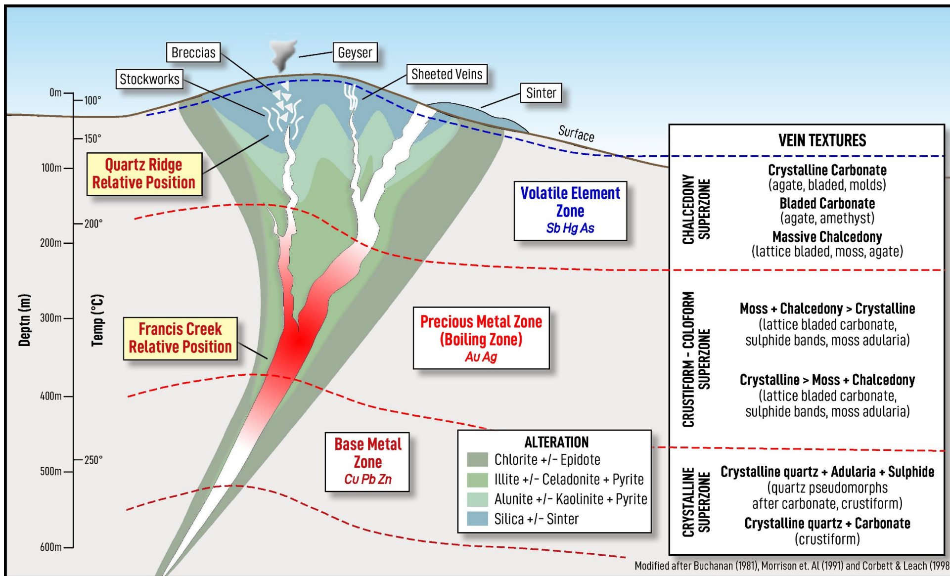
Figure 6: Idealised schematic section through a low sulphidation epithermal system. Drilling at Francis Creek is exhibiting crustiform - colloform – moss textures, sulphide bands and adularia, consistent with the Precious Metal or Boiling Zone depicted above.
