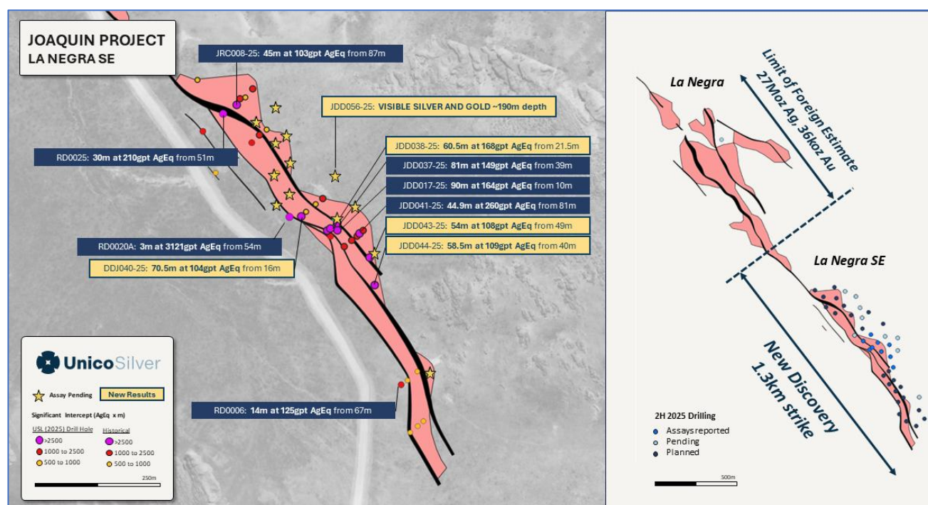
Figure 8: La Negra SE drill hole location
