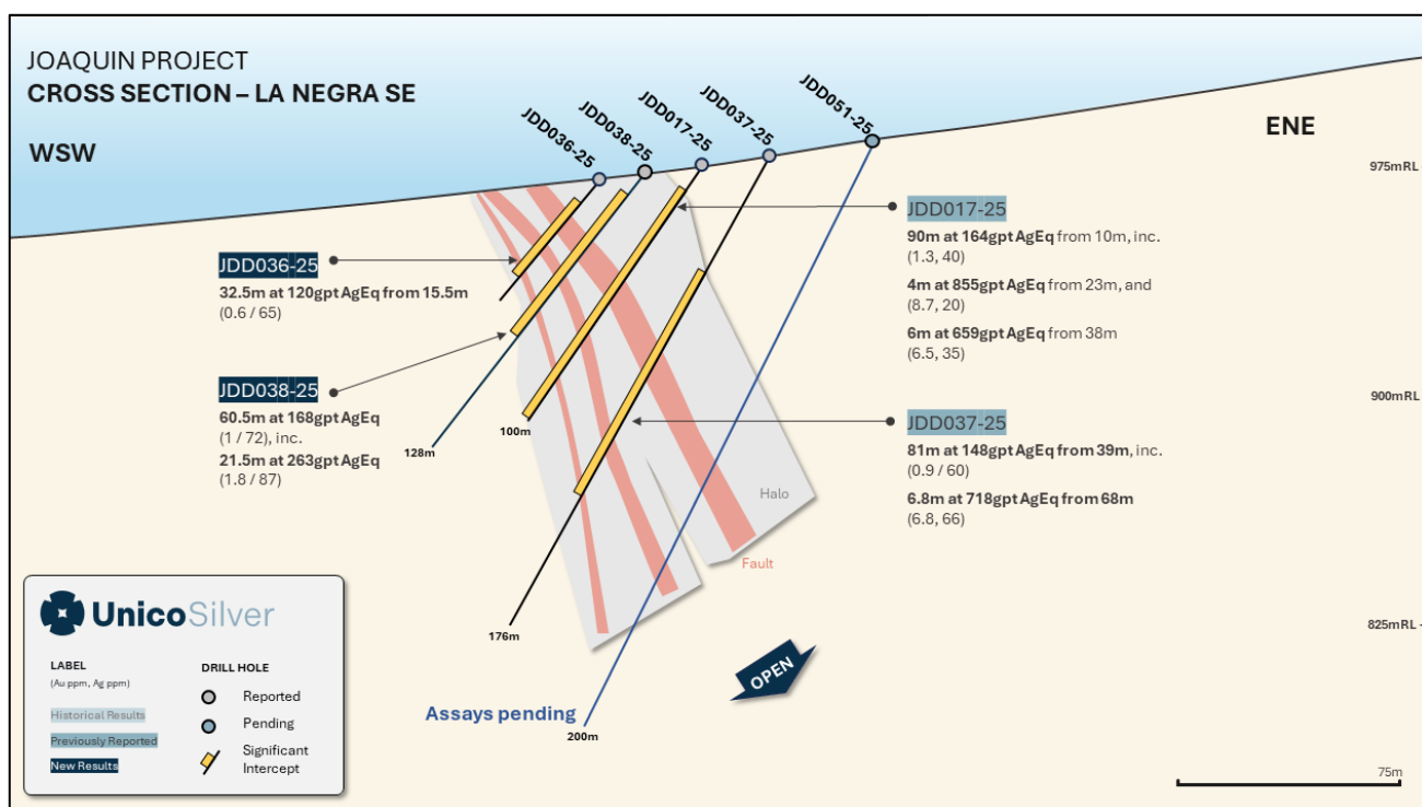
Figure 10: La Negra SE, JDD036-25 and JDD038-25 Cross Section
