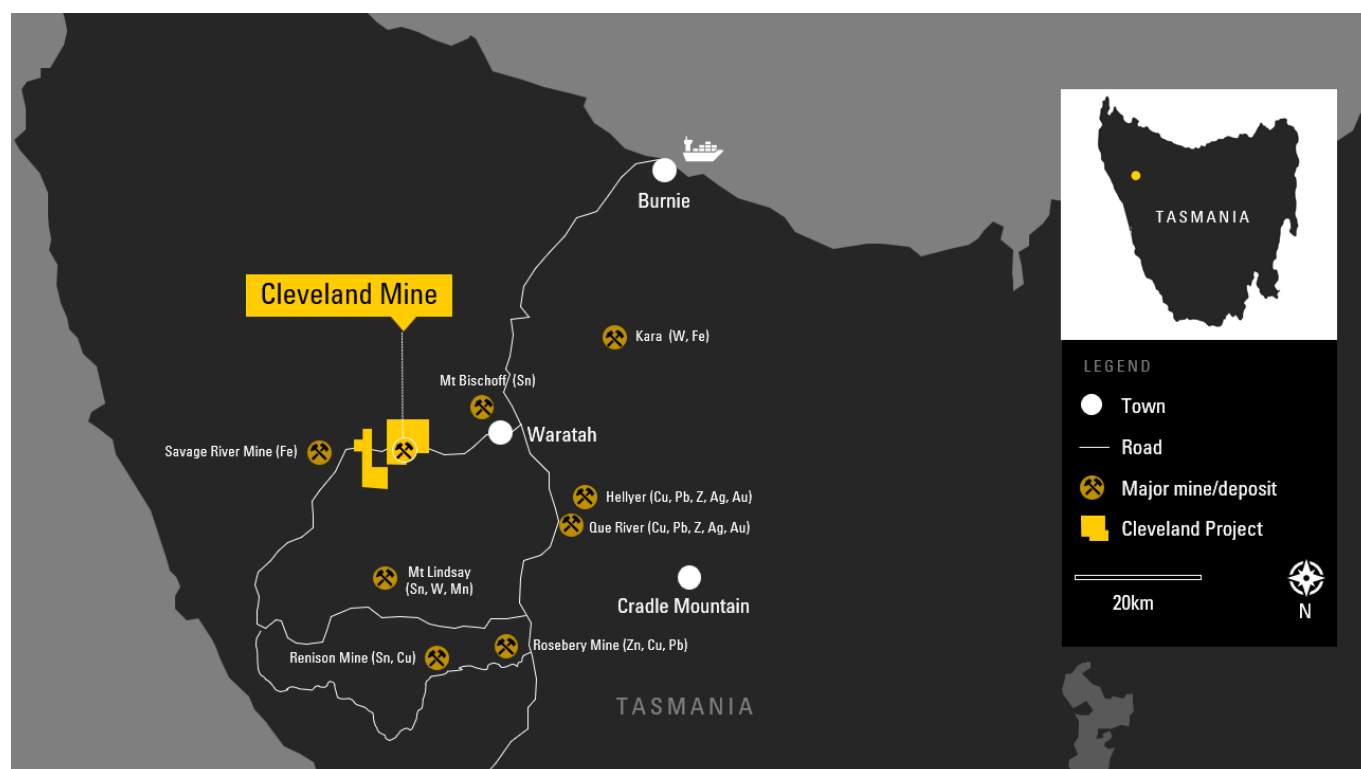
Figure 3. Location of Cleveland Tin Project Tasmania, Australia.
