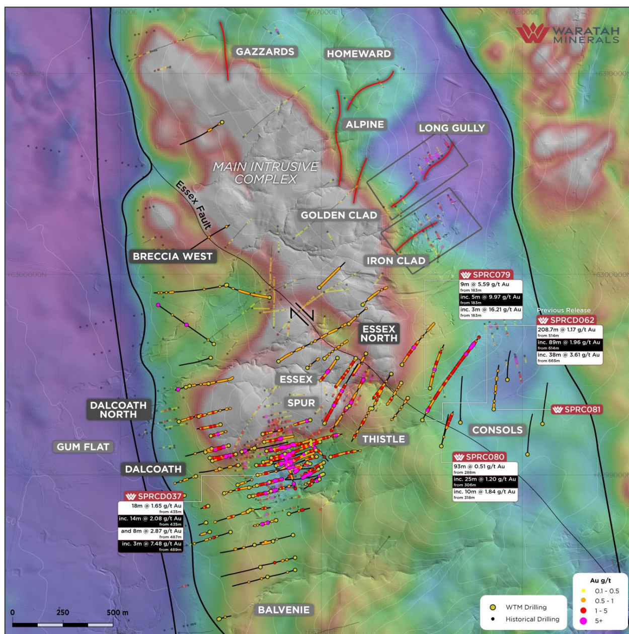
Figure 2: Spur Project, Main Intrusive Complex Targets, Spur Gold Corridor, and other epithermal and porphyry targets, drilling coverage, major surface geochemical trends over RTP magnetics. Ridgeway Deposit outline from Holliday et al 2000
