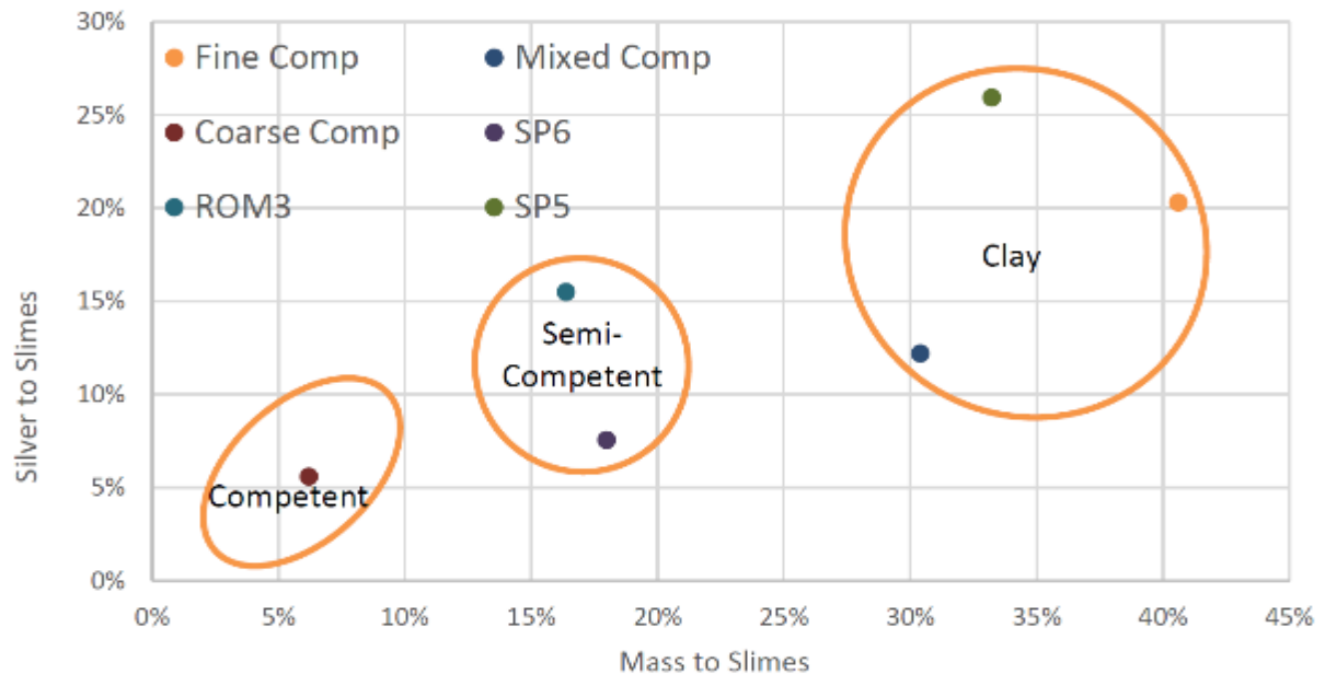
Figure A4: Silver/Mass Department for -38µm fraction of Wonawinta ore.
