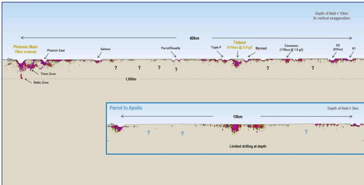
Figure 12: Plutonic gold belt showing limited drilling and areas of the belt untested at depth
