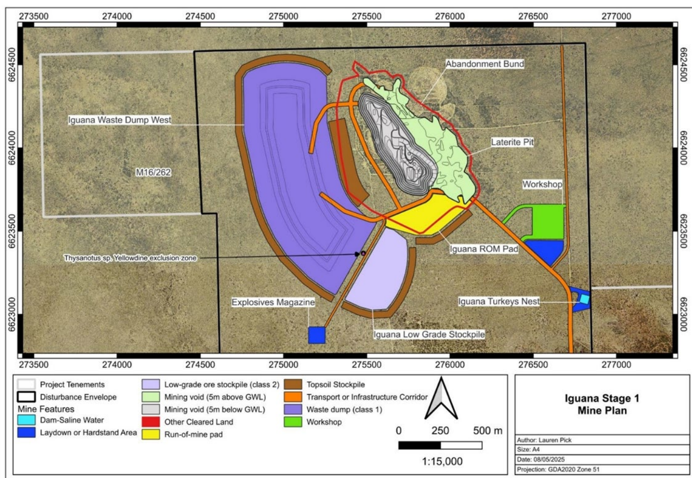
Figure 4: Infrastructure of the Lady Ida Project (Iguana Deposit)
