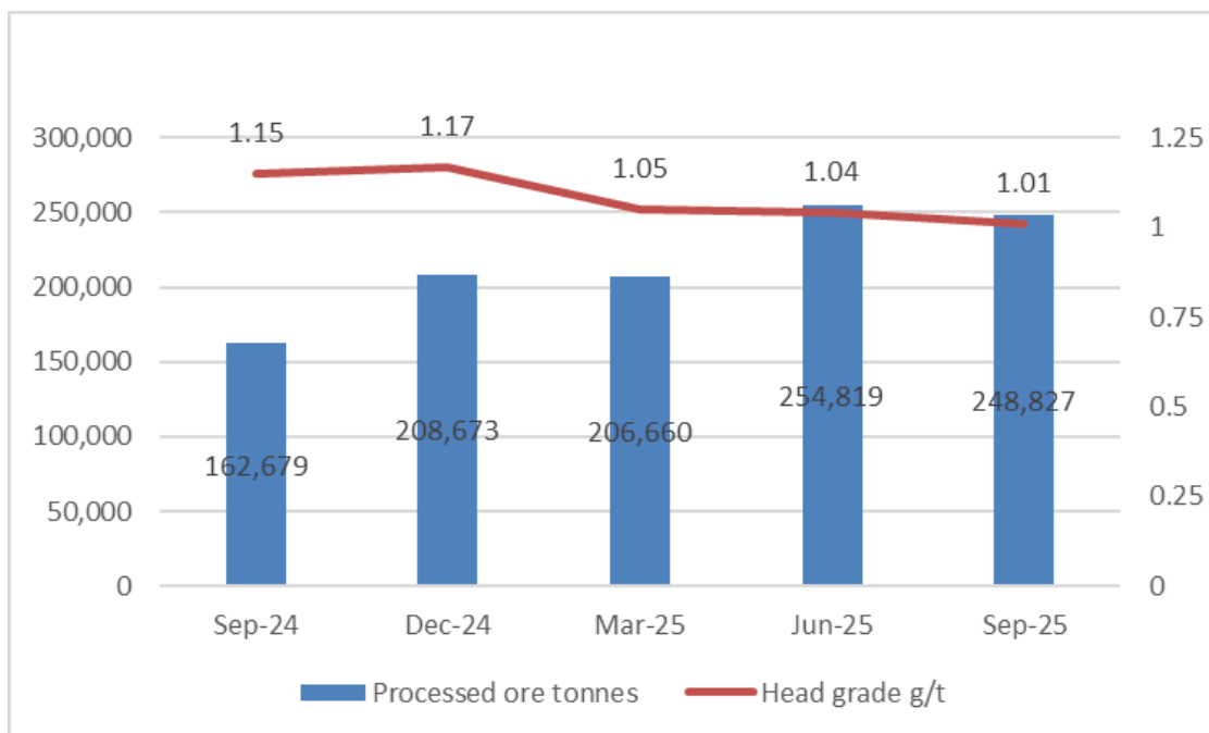
Figure 3: Jaurdi Processed Ore Tonnes and Head Grade
