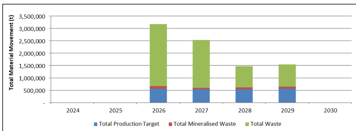
Figure 5-4: Total Material Movement
