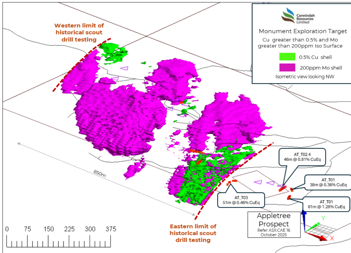
Figure 6: Coincident high grade Cu isosurface +0.5% Cu and Mo isosurface +200ppm at the Monument Exploration Target within the Southern Target Zone. Appletree Dunno Prospect shows clear association whilst the north west is under investigation. (isometric view looking down to NW)
