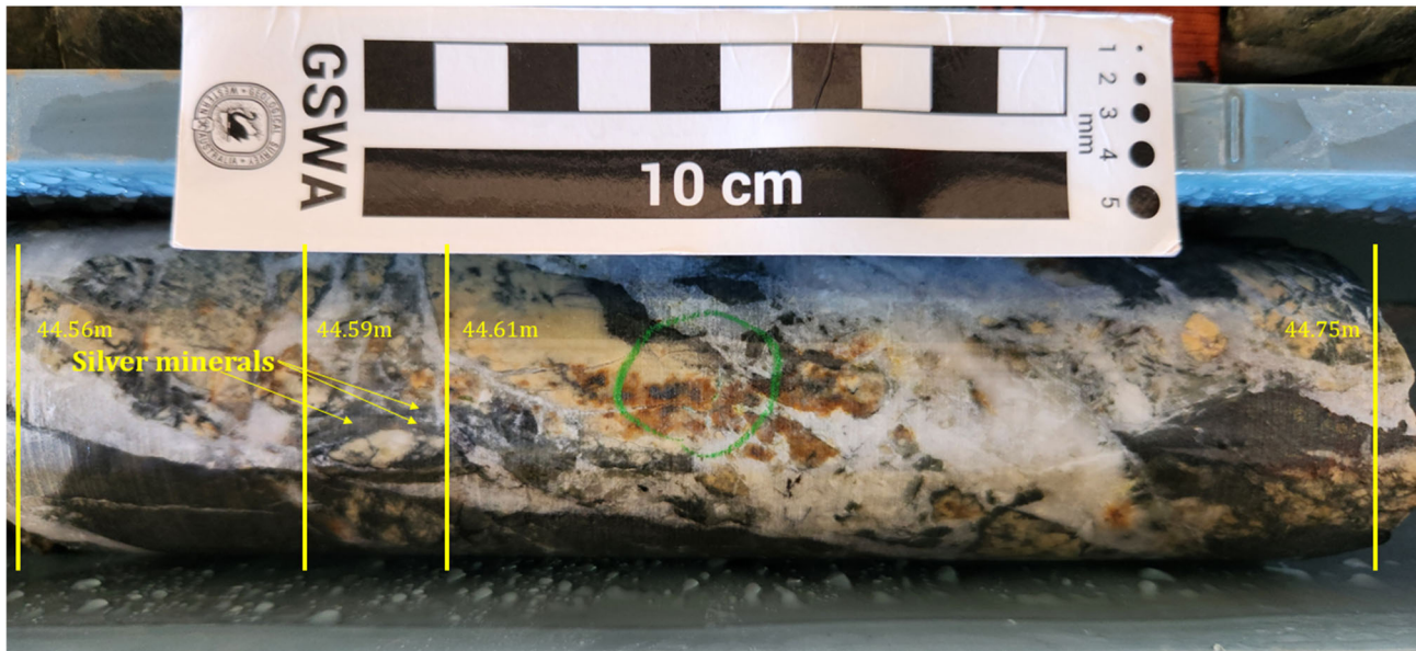
Figure 6. Photograph of HQ3 diamond drill core (25WCDD016) from 44.56m to 44.75m showing several up to 2cm long black minerals from 44.59m to 44.61m forming approximately 1% of the breccia. These minerals are hosted in a carbonate-matrix breccia and pXRF confirmed the presence of silver in the black mineral.
