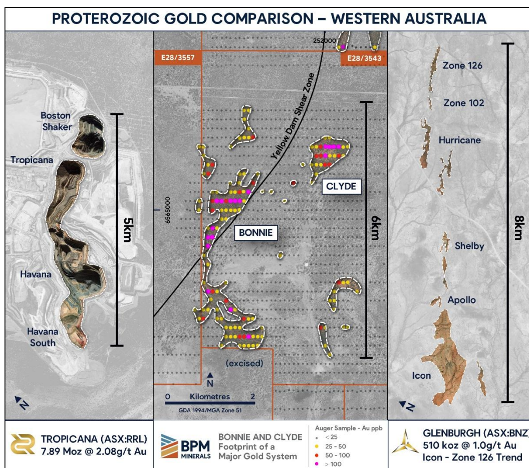
Fig. 3 - Bonnie & Clyde scaled footprint comparison with major WA Proterozoic-hosted gold deposits - Tropicana and Glenburgh
