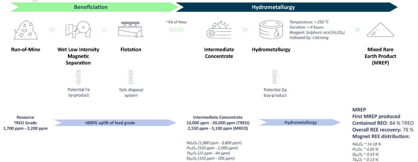
Figure 3: Jupiter beneficiate-first flow sheet now with MREP and Gallium byproduct streams
