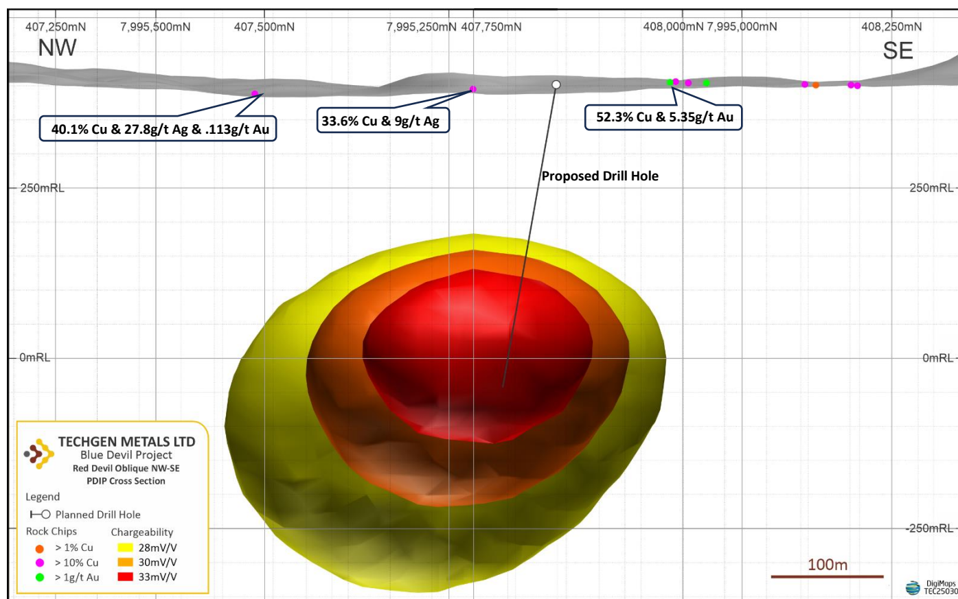
Figure 1: Red Devil 3D IP inversion model with surface rock chips shown. Planned drill hole trace shown.
