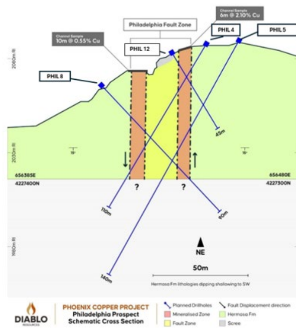
Figure 5 - Philadelphia Prospect-Cross Section Looking NE
