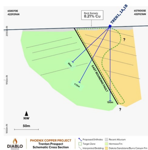
Figure 3 - Trenton Prospect Cross Section Looking NW
