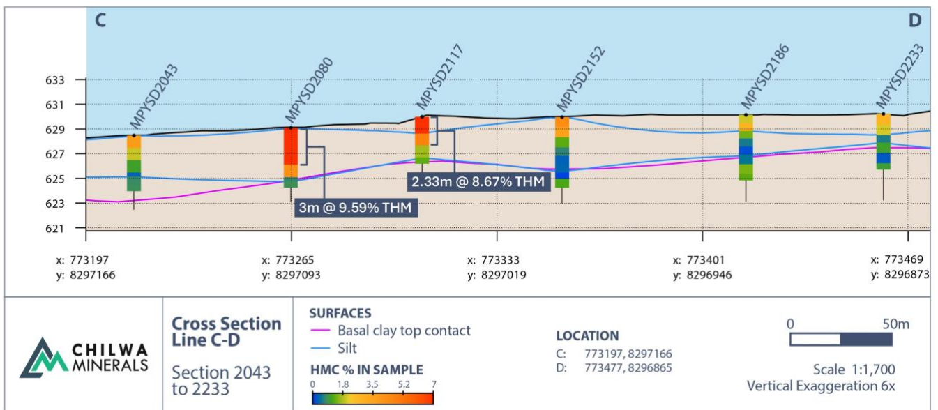
Figure 3: Cross section C-D (ref Figure 1), Mpyupyu Flats North MPYSD2043 to MPYSD2233.
