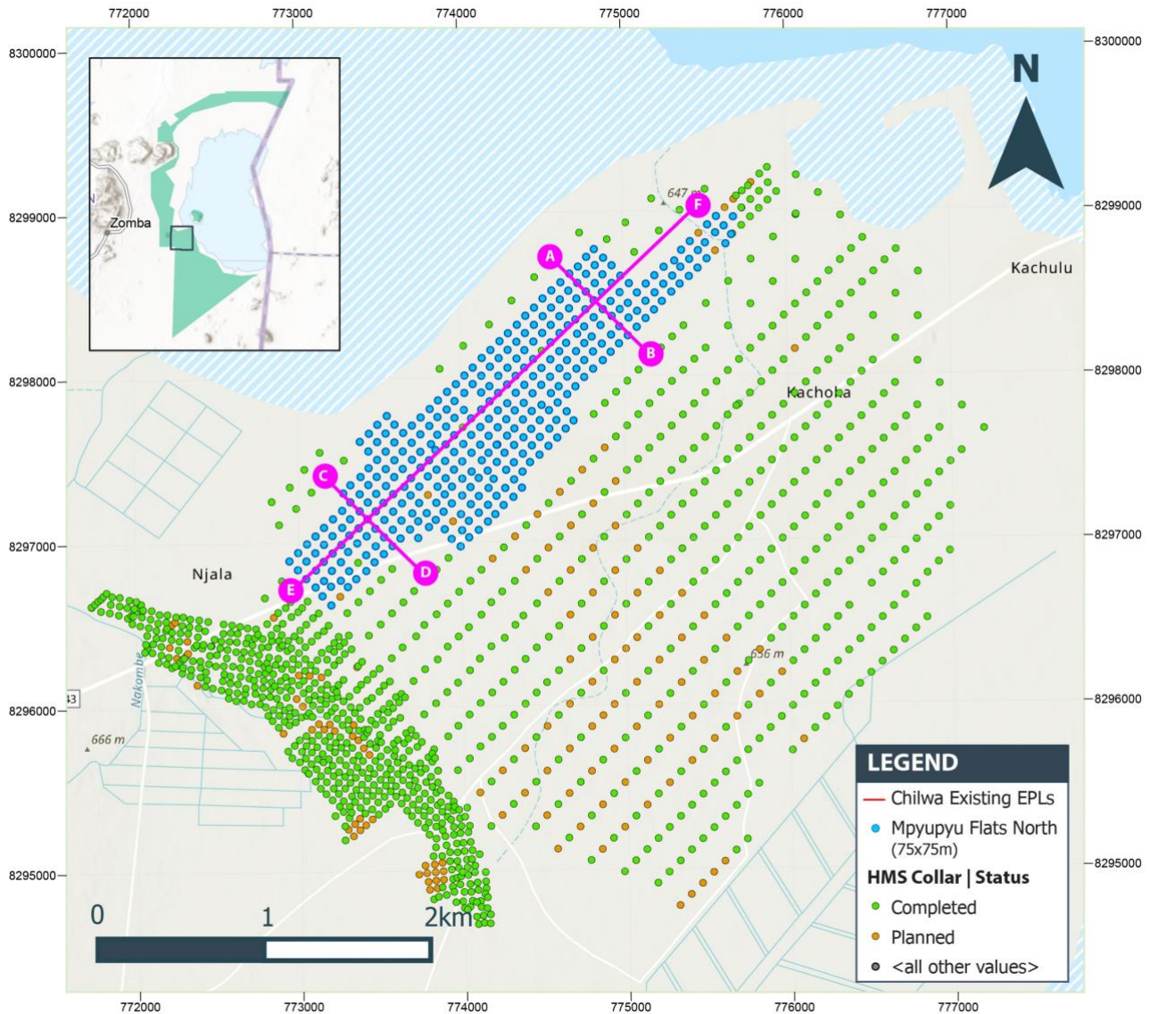
Figure 1: Mpyupyu Dune (west/left) and Mpyupyu Flats deposits. Results are presented for an area to the north of Mpyupyu Flats (blue circles)
