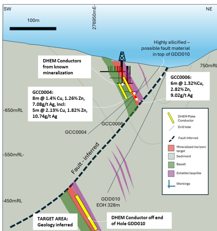
Figure 1: Cross-section SE-NW across Gulf Creek showing plate conductors
