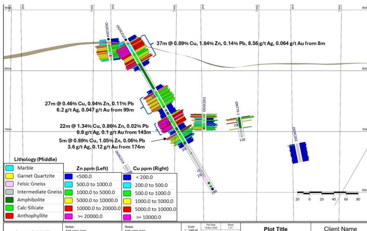
Figure 2. Drillhole cross section showing the four main mineralised zones within OGR010 with a combined length of 91m (looking southeast, 20m section window).
