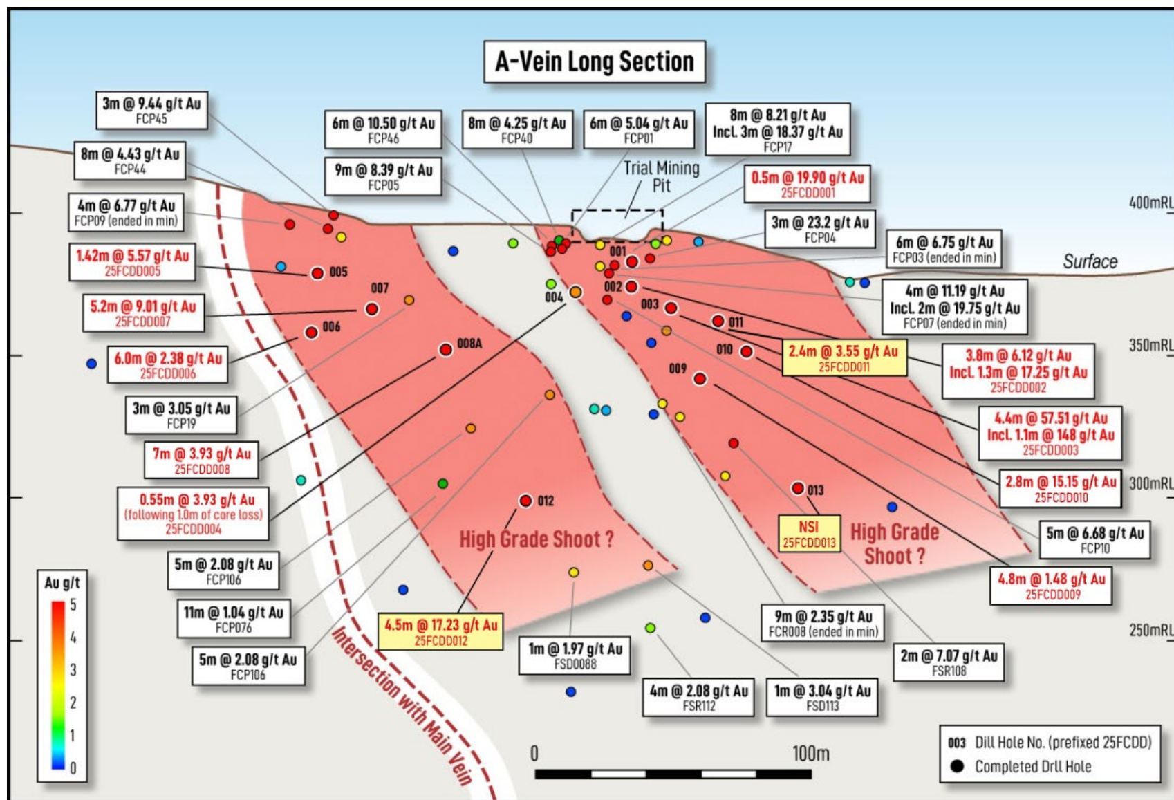
Figure 3: A-Vein long section with historic significant intercepts (white), current drilling pierce points and latest assay results (yellow).
