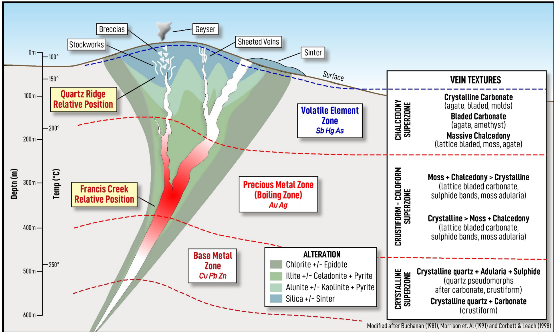
Figure 2: Idealised schematic section through a low sulphidation epithermal system. Drilling at Francis Creek is exhibiting crustiform - colloform – moss textures, sulphide bands and adularia, consistent with the Precious Metal or Boiling Zone depicted above.
