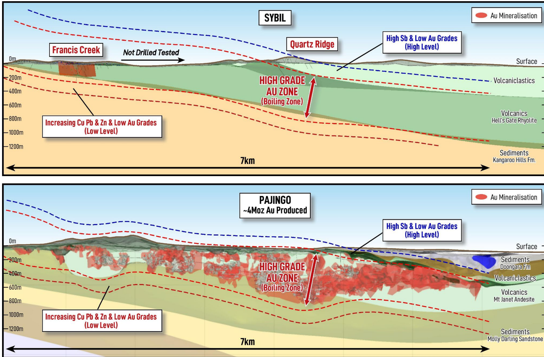
Figure 5: Schematic comparison of the Sybil and Pajingo epithermal systems (both long sections are looking north). Figure modified from AIG NEQ Minerals Workshop Presentation, "Pajingo – exploring undercover", March 2022.
