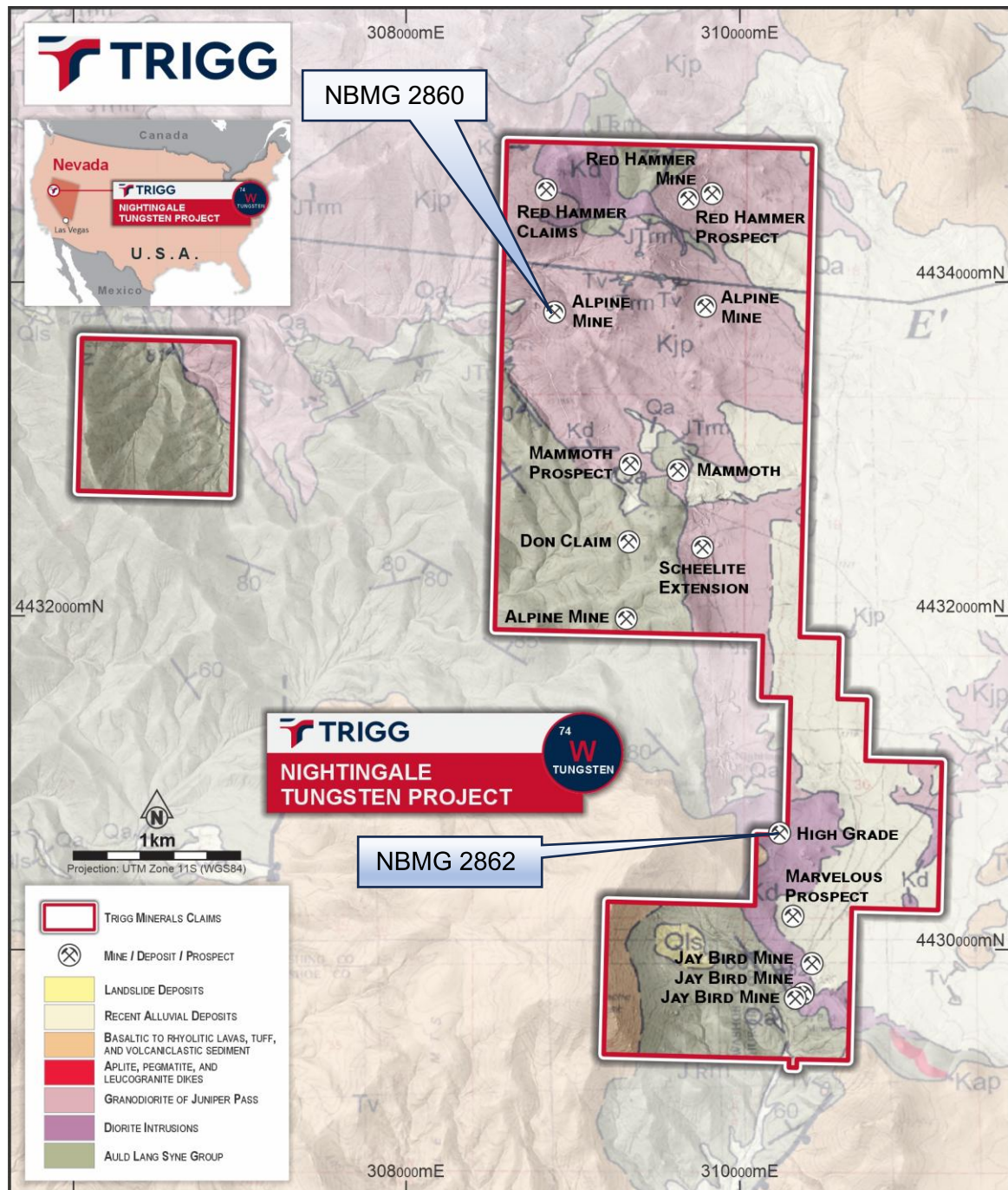
Figure 3. Nightingale Project location, claim area and rock chip sample locations showing the historical mines and prospects over the geology.
