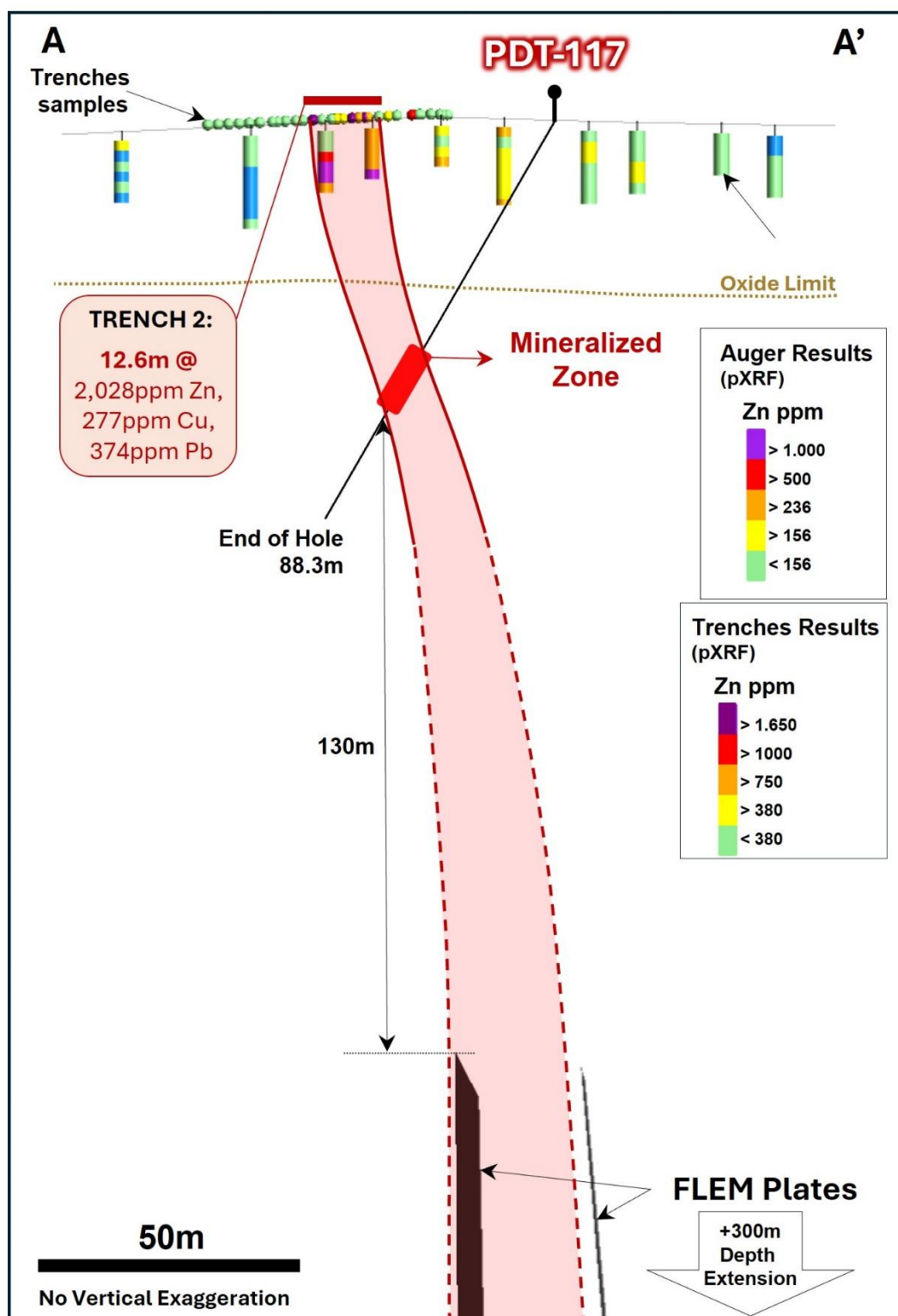
Figure 3: Touro cross section through Trench 2 and PDT117. A mineralised zone of 13m from 54m downhole was intercepted.
