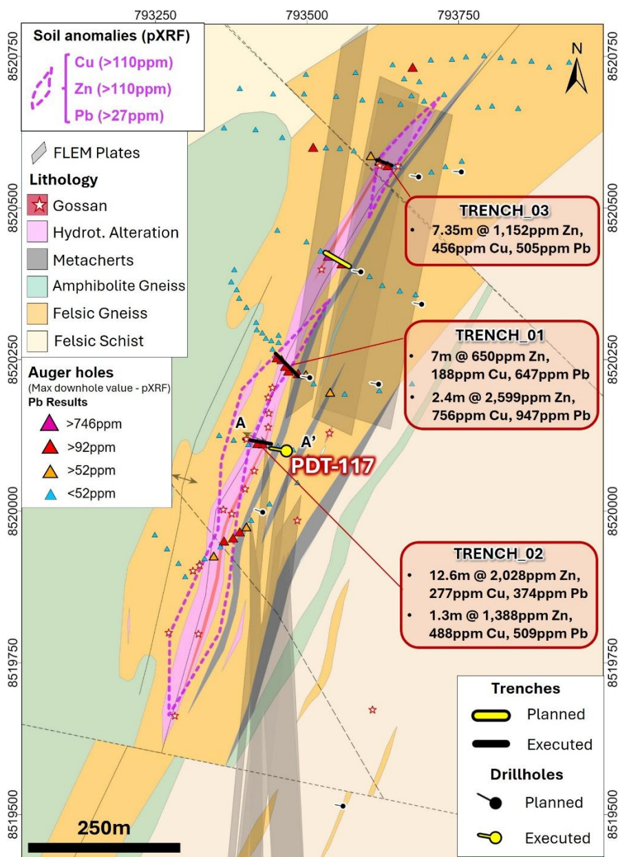
Figure 2: Touro Prospect plan, first hole of the current campaign- PDT_117 which intersected massive sulphide mineralisation. Trench locations, geochemical anomaly, gossans and the hydrothermal alteration zone.
