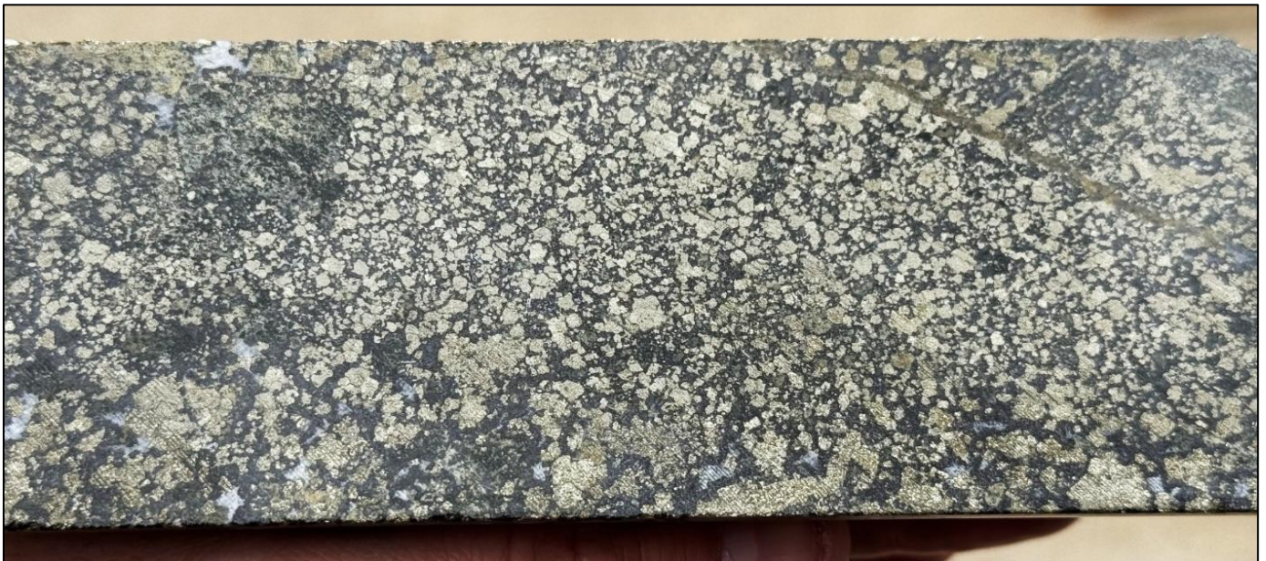
Figure 6: Core photo of replacement-type, chlorite-silica-magnetite altered green garnet skarn with semi-massive sulphide in ZRSD25217 – 496.7m to 498.7m – 16.5g/t AuEq 2 (15.6g/t Au, 0.3% Cu, 0.2% Pb, 0.1% Zn & 12.6g/t Ag).
