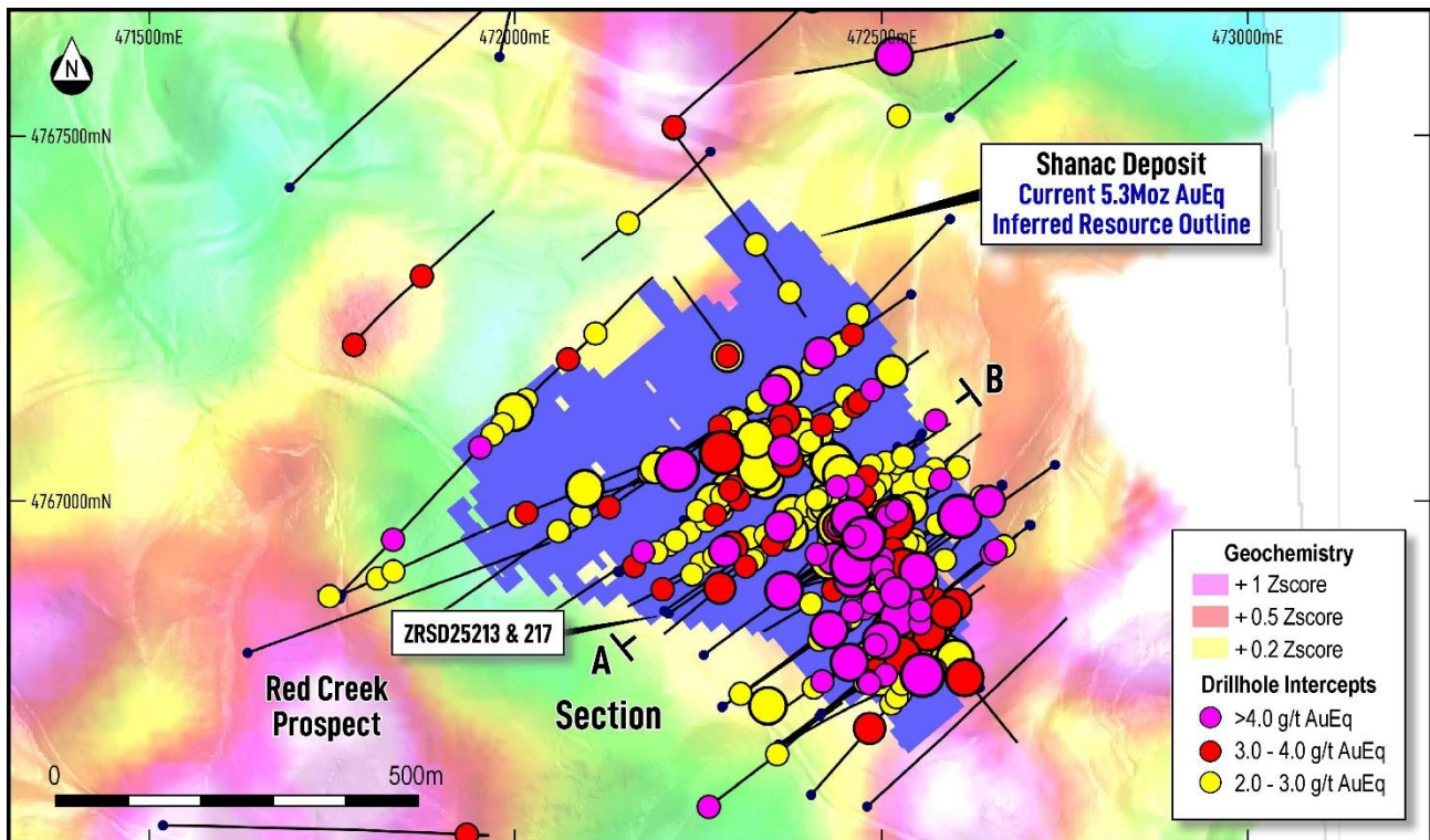
Figure 2: Plan view map of the Shanac deposit, showing the resource footprint, drill-hole collars and traces, high-grade intercept points and background Au-As in soil geochemistry.
