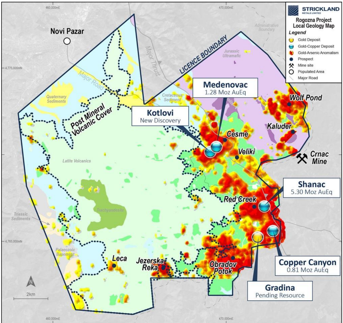
Figure 1: Plan view map of the Rogozna Project, showing geology with deposits, prospects and geochemical anomalism.
