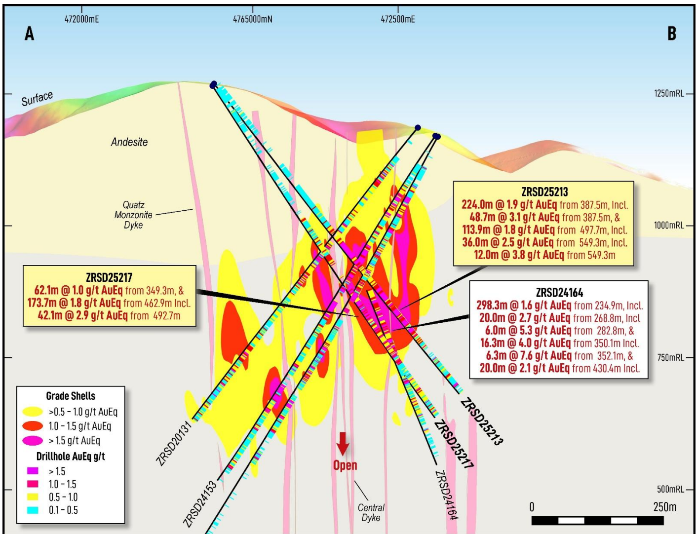
Figure 4: Shanac cross-section view looking NW (50m view width), showing drill-hole traces with intercepts, geology, AuEq grade shells and the new copper-gold zone with prospective search space.
