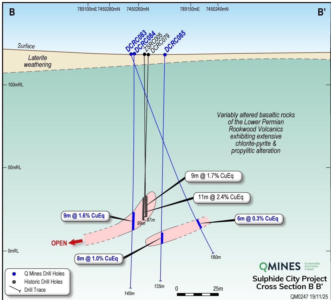
Figure 4: Cross-section through B-B' looking NE. Section window if +/- 12.5m
