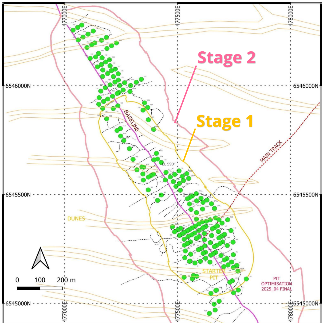
Fig. 2 – Tunkillia S1 & S2 optimised open pit outlines with completed Phase 1 drilling (green dots)
