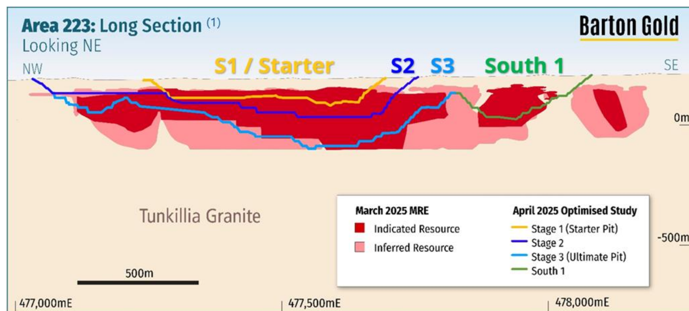
Fig. 1 - Long section showing Area 223 'Main' pit and stages, and Tunkillia JORC MRE block model 1
