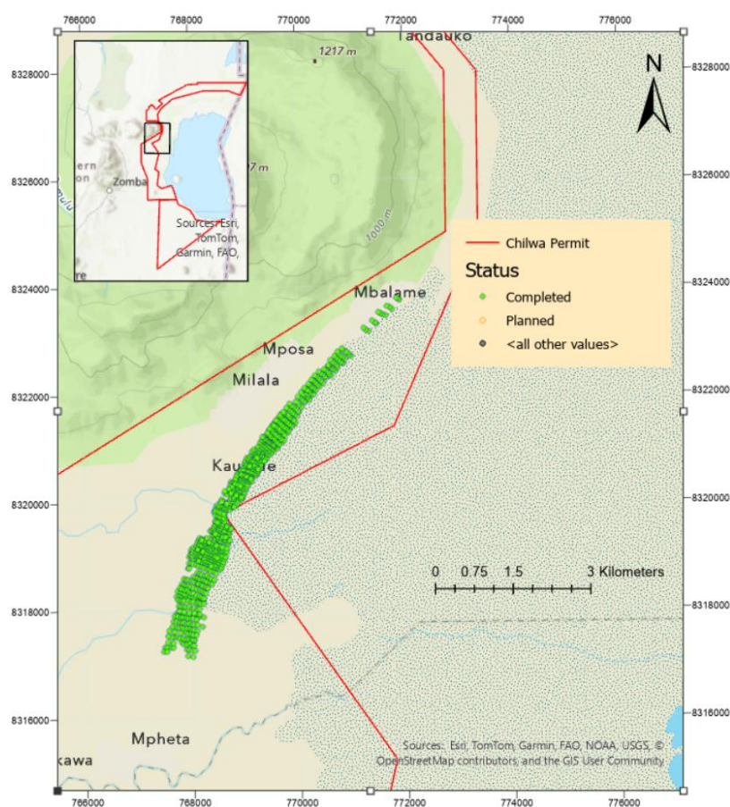
Figure 3 Sonic drilling points at the Mposa Deposit
