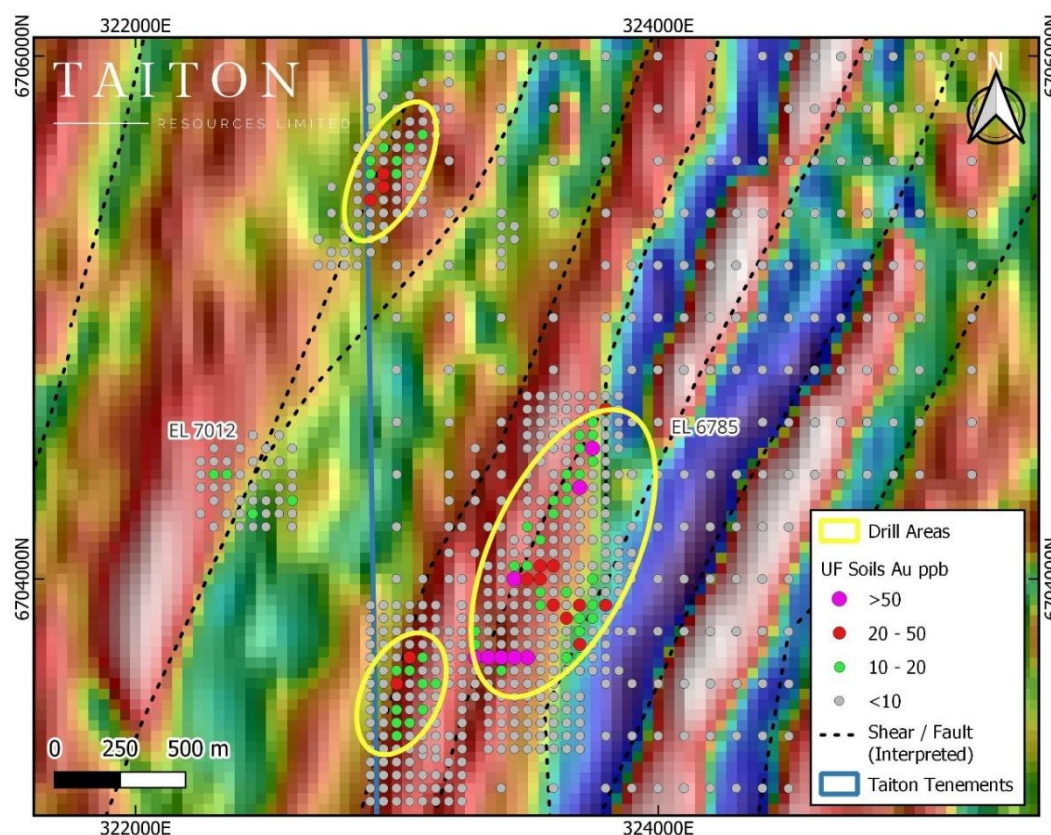
Figure 3 Challenger West Area 1 UF soil results underlain by RTP IVD magnetic image.
