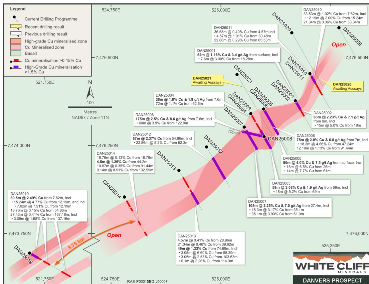
Figure 5 - Plan view of 2025 Spring and Summer RC drillholes at the Danvers Breccia System showing surface projection of intercepted mineralisation. Assay results included in this announcement are shown at E (DAN25010, DAN25011 Figure 3) and G (DAN25014, Figure 2).
