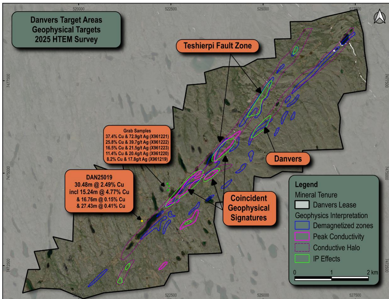
Figure 3 - Satellite image with polygons of geophysical signatures which are overlapping in several locations to produce robust geophysical targets with similar signatures to Danvers.
