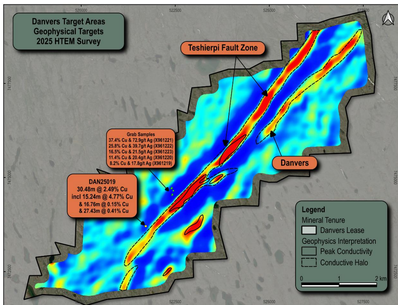
Figure 1 - Map of early time EM channels X component, RGB of 3 channels converted to single band pseudo-colour. Red areas represent peak conductivity highlighted by thicker black lines within a halo of conductivity, thinner dashed lines.
