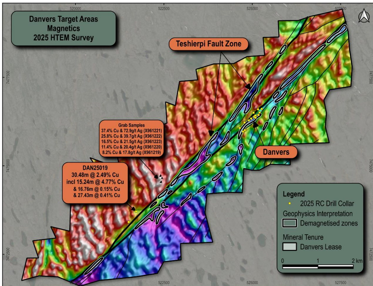
Figure 2 - Total Magnetic Intensity map, highlighting zones of demagnetisation along prospective NE/SW trending faults.
