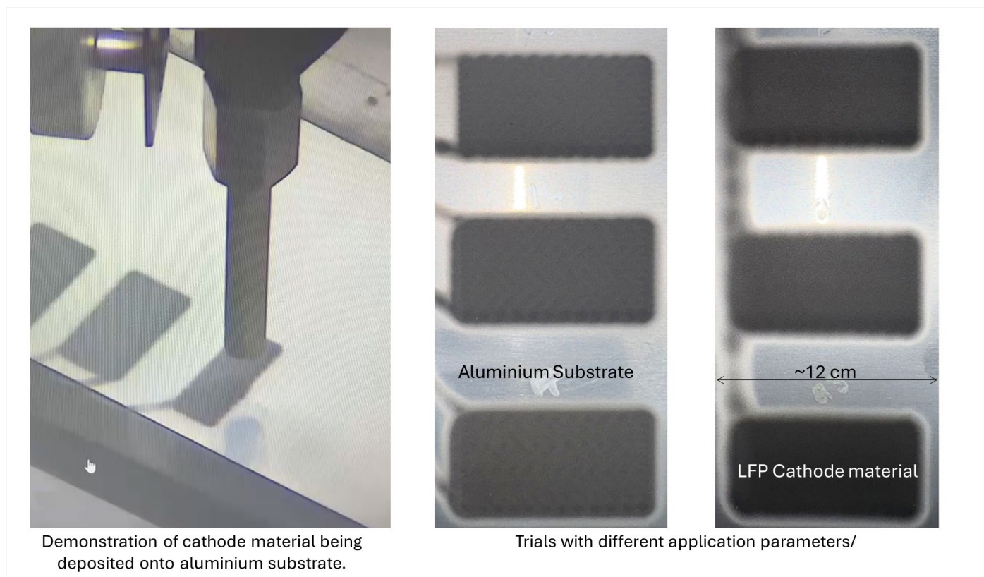
Figure 1 – Early successful tests of dry-supersonic-deposition (DSD) of Lithium-Iron-Phosphate (LFP) cathode material onto battery pouch cell aluminium foil substrate.
