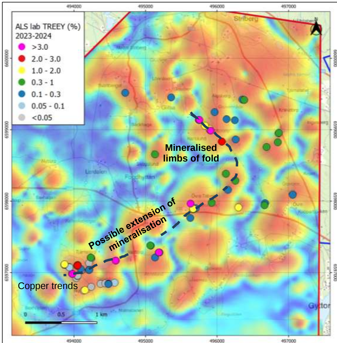
Figure 2: Locations of Bastion rock chip samples, showing REE results and observations in the north of the Gyltorp property (refer to Figure 1 for the overview location). The figure includes recent samples and some samples from late 2023 sampling by Bastion.
