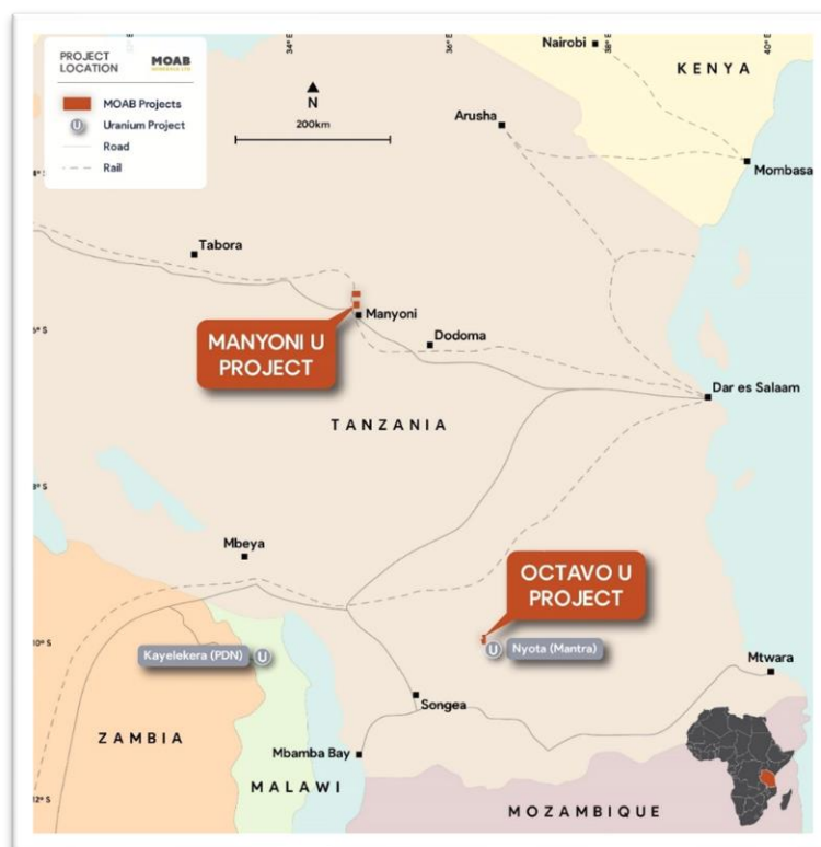
Figure 1. Location of Manyoni and Octavo Uranium Projects
