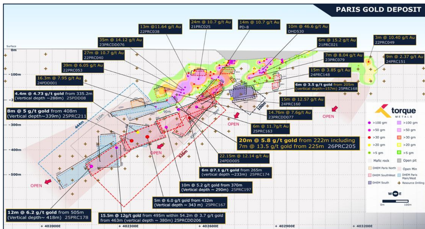
Figure 1 Paris gold deposit, drilling program and DHEM plates indicating extensions beyond existent MRE
