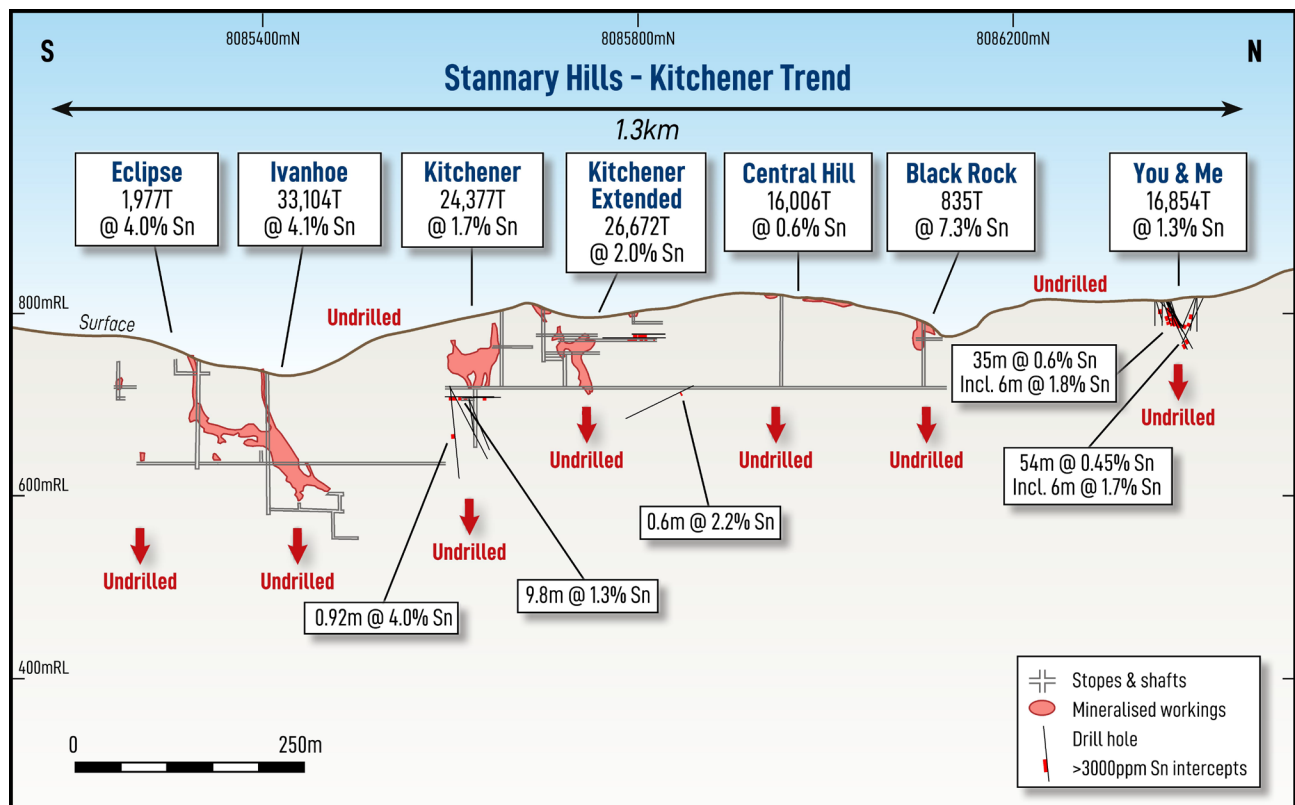
Figure 4: Long section showing a group of seven high-grade mines over 1.3km of strike along the Kitchener Trend and the very limited drilling completed, both between historical mines and at depth
