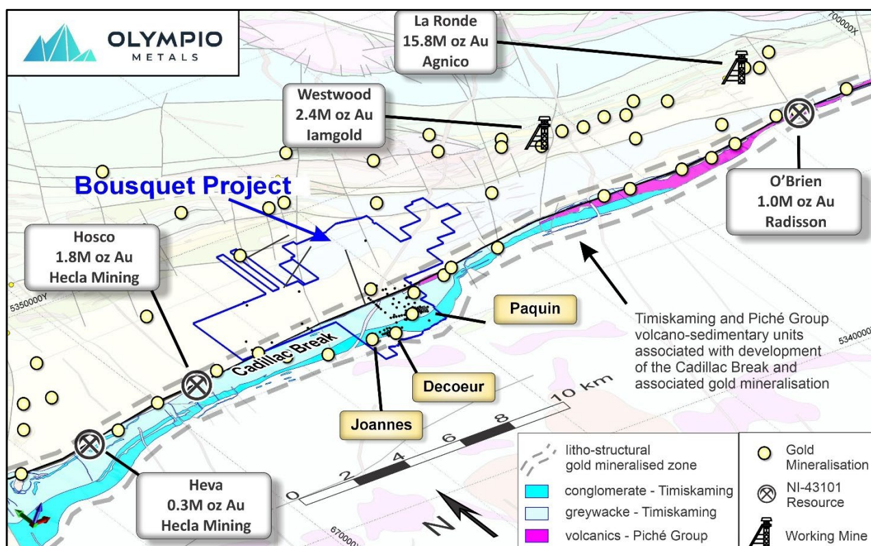
Figure 2: Litho-structural setting of the Bousquet project with nearby gold resources
