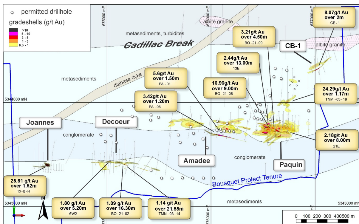
Figure 4: Mineralised structures and selected intervals within advanced gold prospects, Bousquet Project
