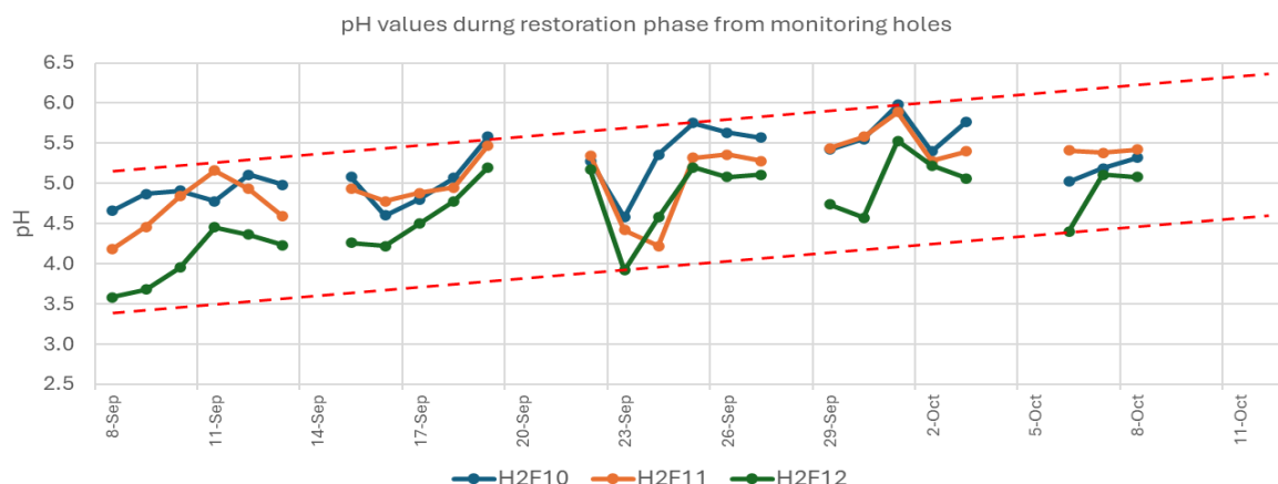
Figure 1. pH measurement values from restoration phase. Water solution extracted from monitoring holes H2F10, H2F11 and H2F12. Local river water at approximately pH7 was injected into the clays during the restoration phase.
