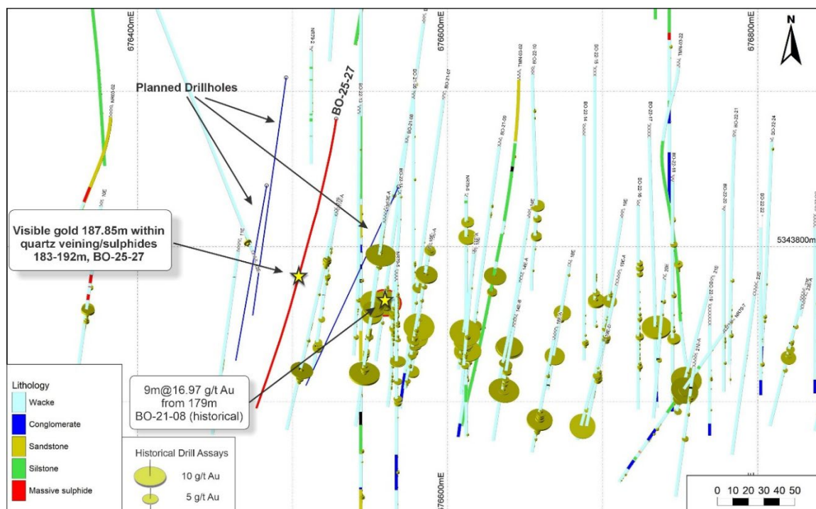
Figure 3: Collar plan of Paquin prospect, showing historical gold assays and hole BO-25-27 visible gold intercept
