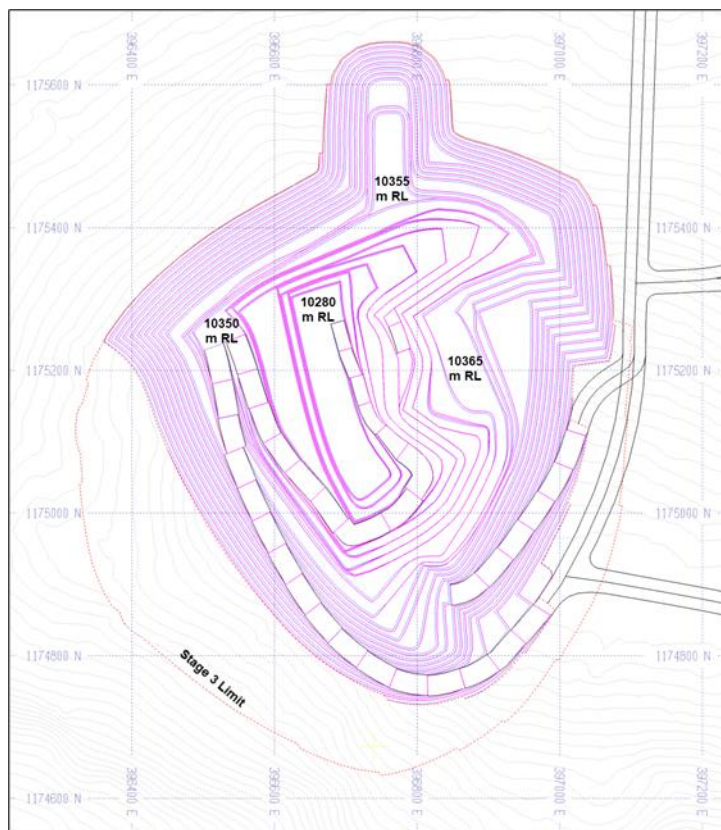
Figure 8.3: NEB Pit Stage 2 Layout
