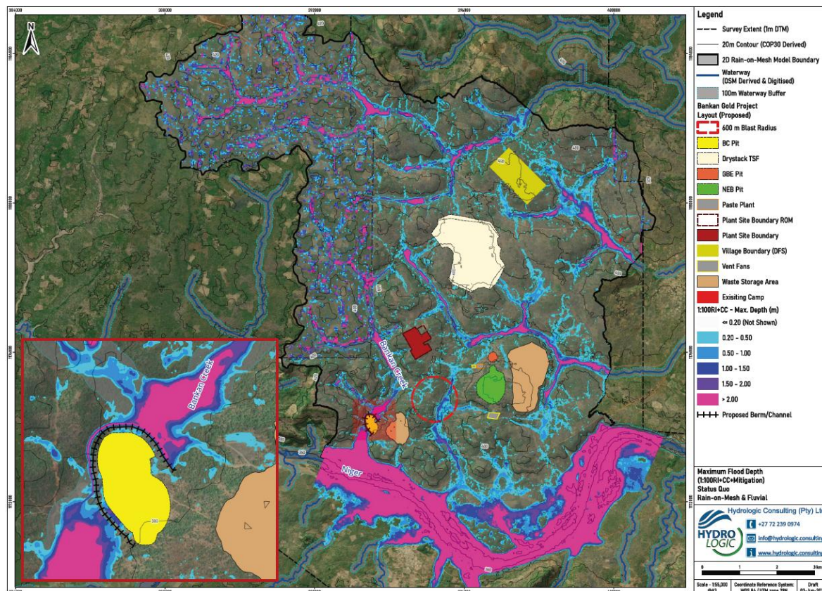
Figure 6.1: Flood Modelling Outcomes 1:100 RI plus Climate Change Event
