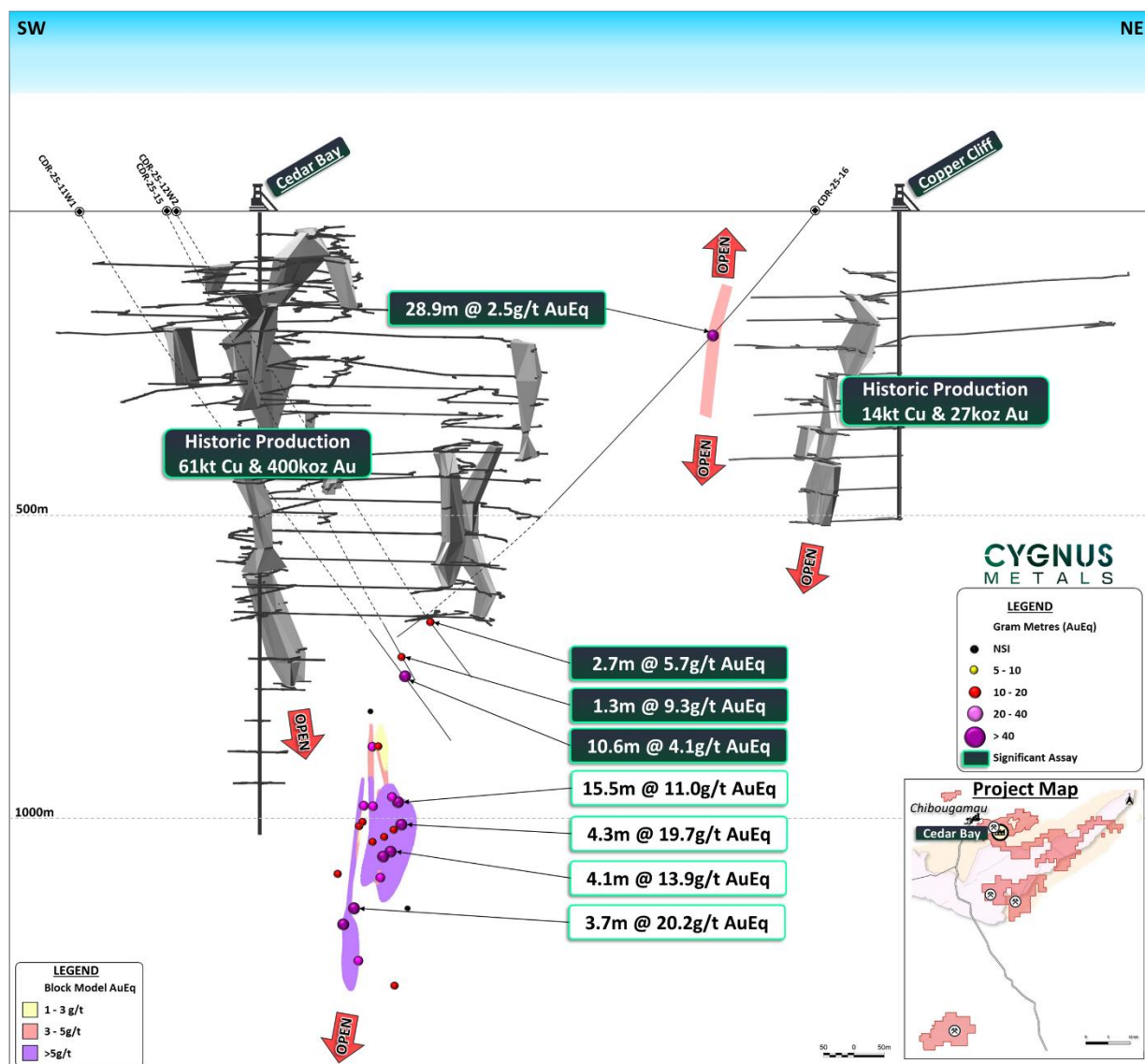
Figure 1: Potential new zone of mineralisation, returning 28.9m @ 2.5g/t AuEq between Cedar Bay 4 and Copper Cliff. All lodes remain open.
