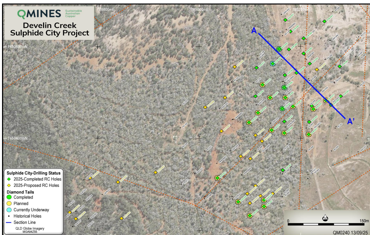
Figure 2: Plan view showing drillhole assay status, collar locations with completed and planned drillholes at Sulphide City.
