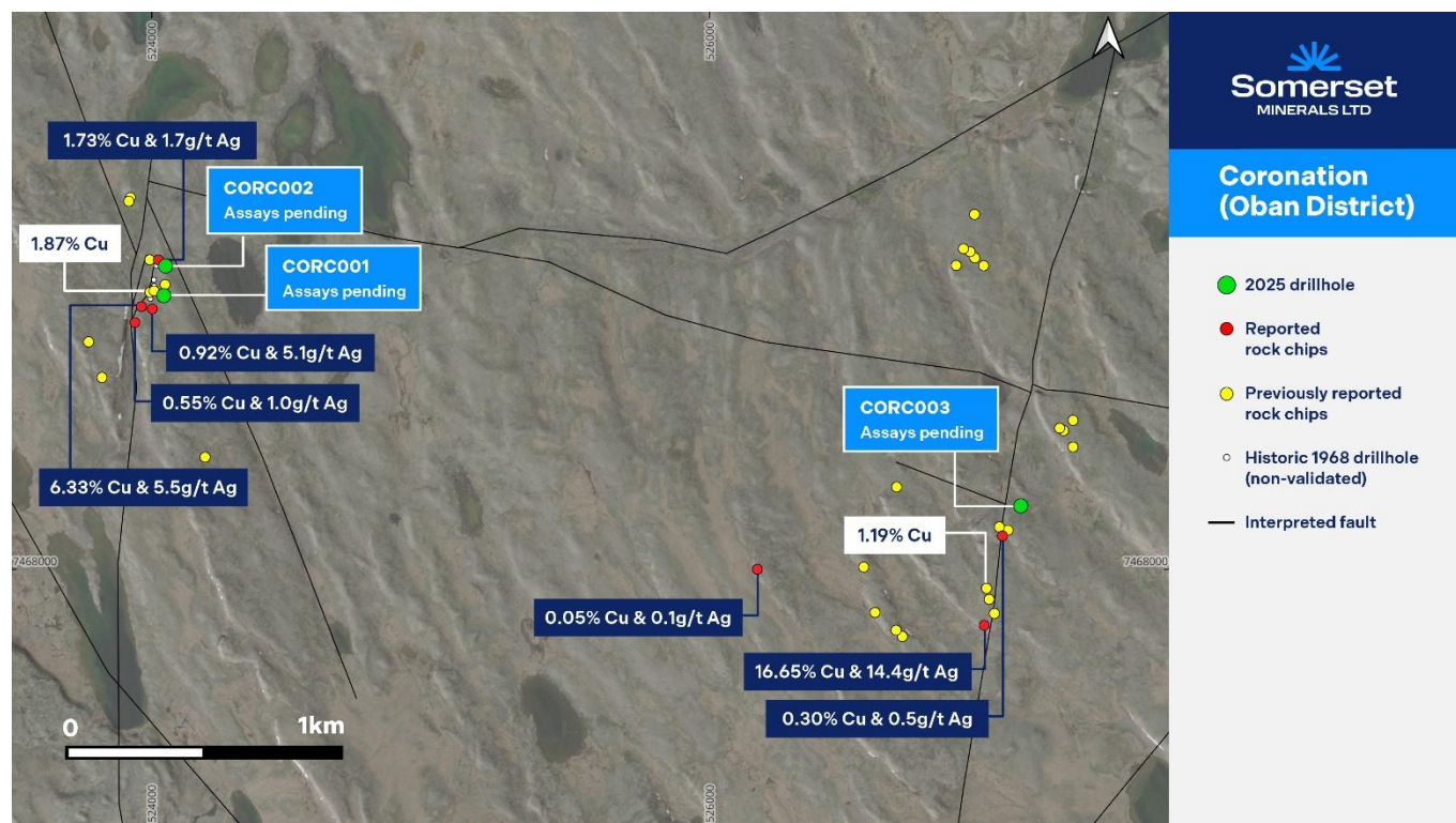
Figure 6: Detailed map of the Coronation target within the Oban District, showing recently received rock chip sample locations.
