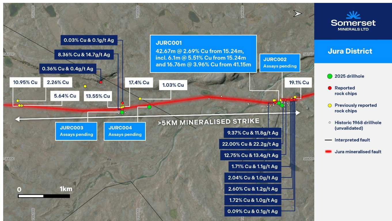
Figure 4: Prospect scale map highlighting new rock chip results across the Jura District, confirming over 5km of continuous copper mineralisation.
