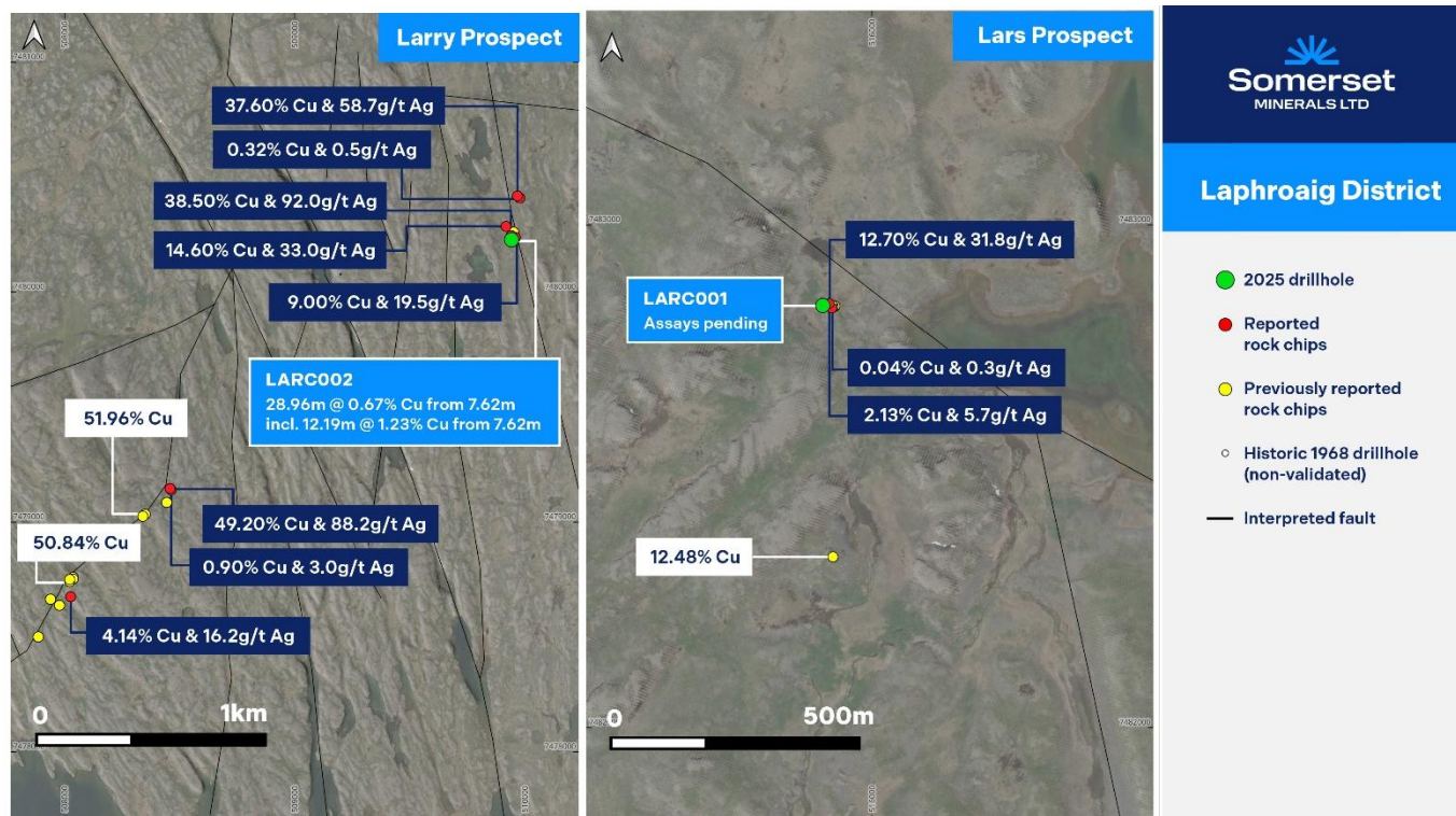
Figure 3: Prospect-scale maps of the Larry and Lars prospects within the Laphroaig District, highlighting newly reported high-grade surface samples.
