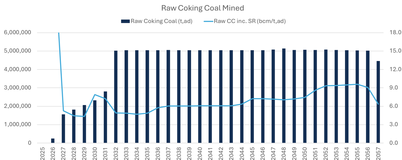
Figure 11. Schedule of Coking Coal Mined (t,ad) per annum
