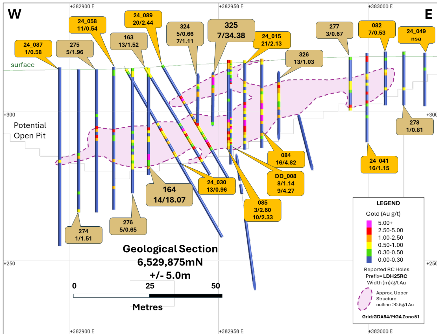
Figure 4: Section 6,529,875mN (looking north +/- 5m) illustrating the results reported today (gold call-outs) and prior reported results (orange call-outs).
