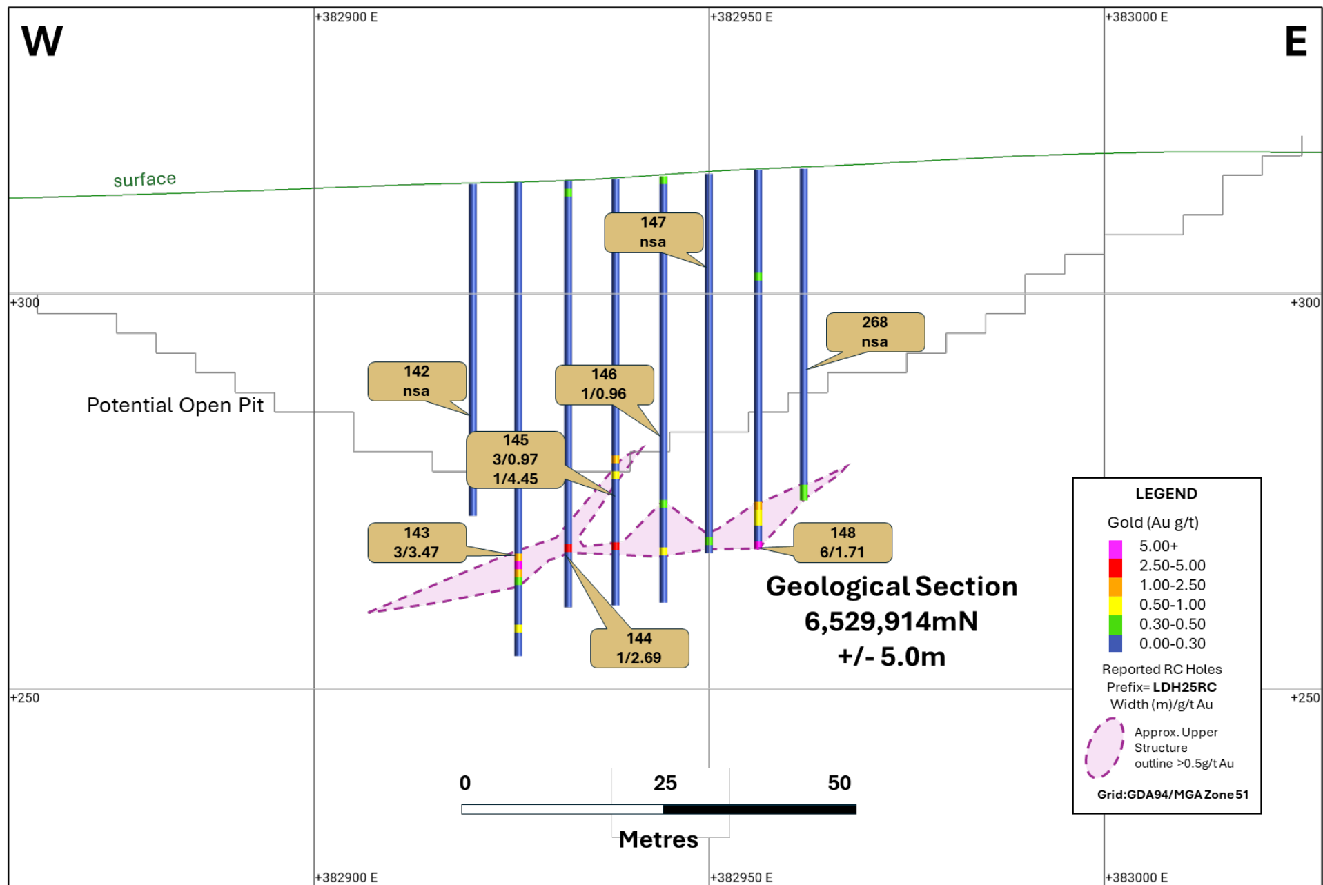
Figure 8: Section 6,529,914mN (looking north +/- 5m) illustrating the results reported today (gold call-outs).
