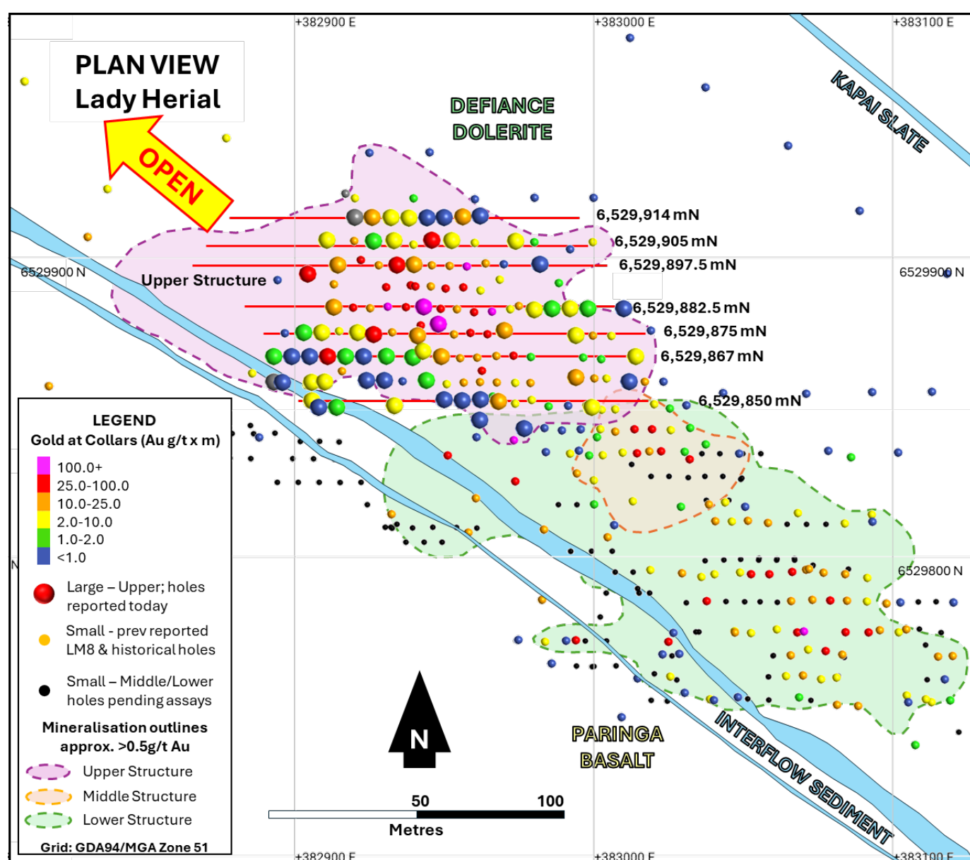
Figure 1: Plan View of the Upper Structure at Lady Herial showing recent grade control spaced results and the section numbers and locations of Figures 2 through 8.
