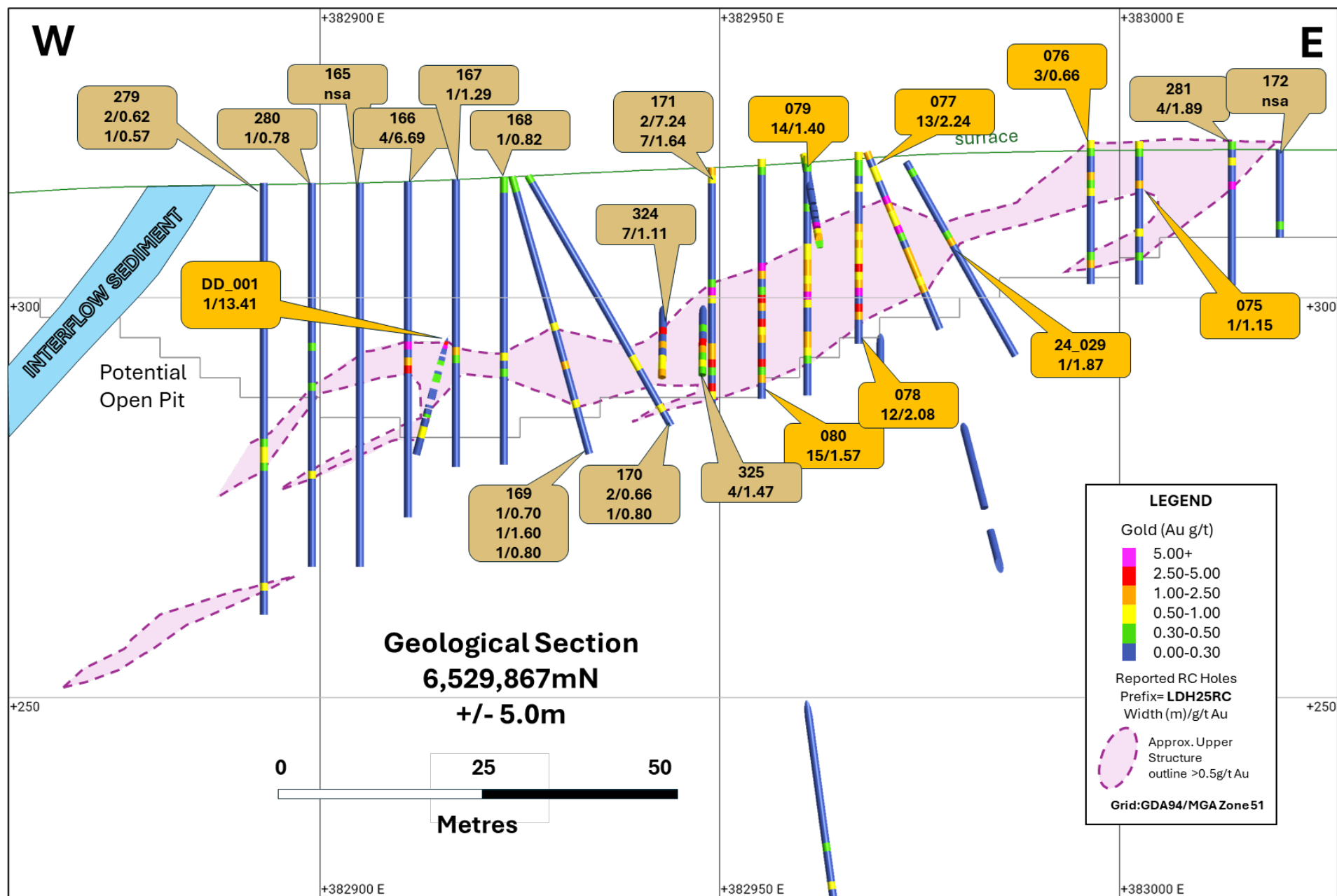
Figure 3: Section 6,529,867mN (looking north +/- 5m) illustrating the results reported today (gold call-outs) and prior reported results (orange call-outs).
