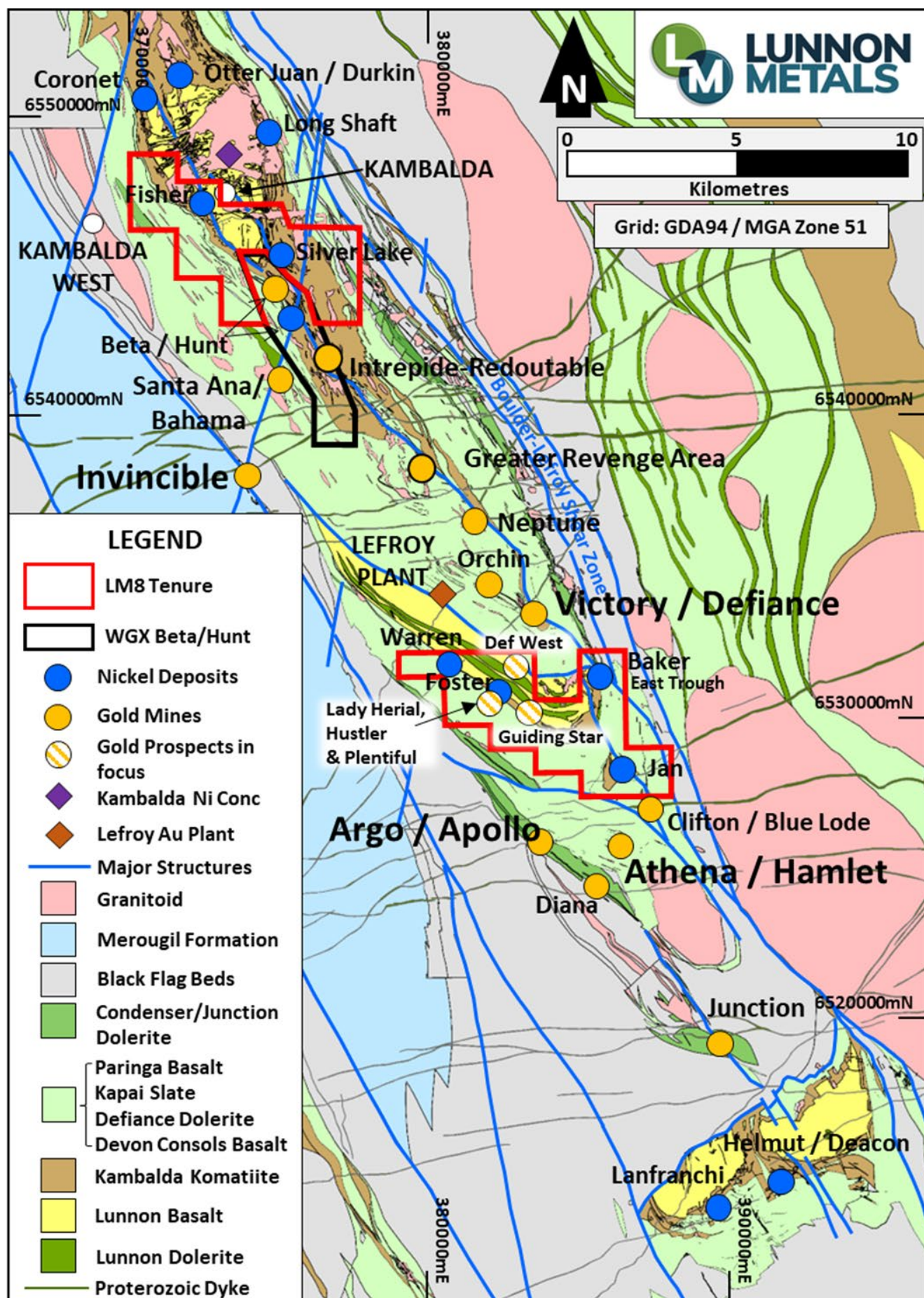
Figure 10: Location of the KGNP (red outlines) at the local Kambalda/St Ives scale; showing surface geology and structure of this significant Australian gold camp.
