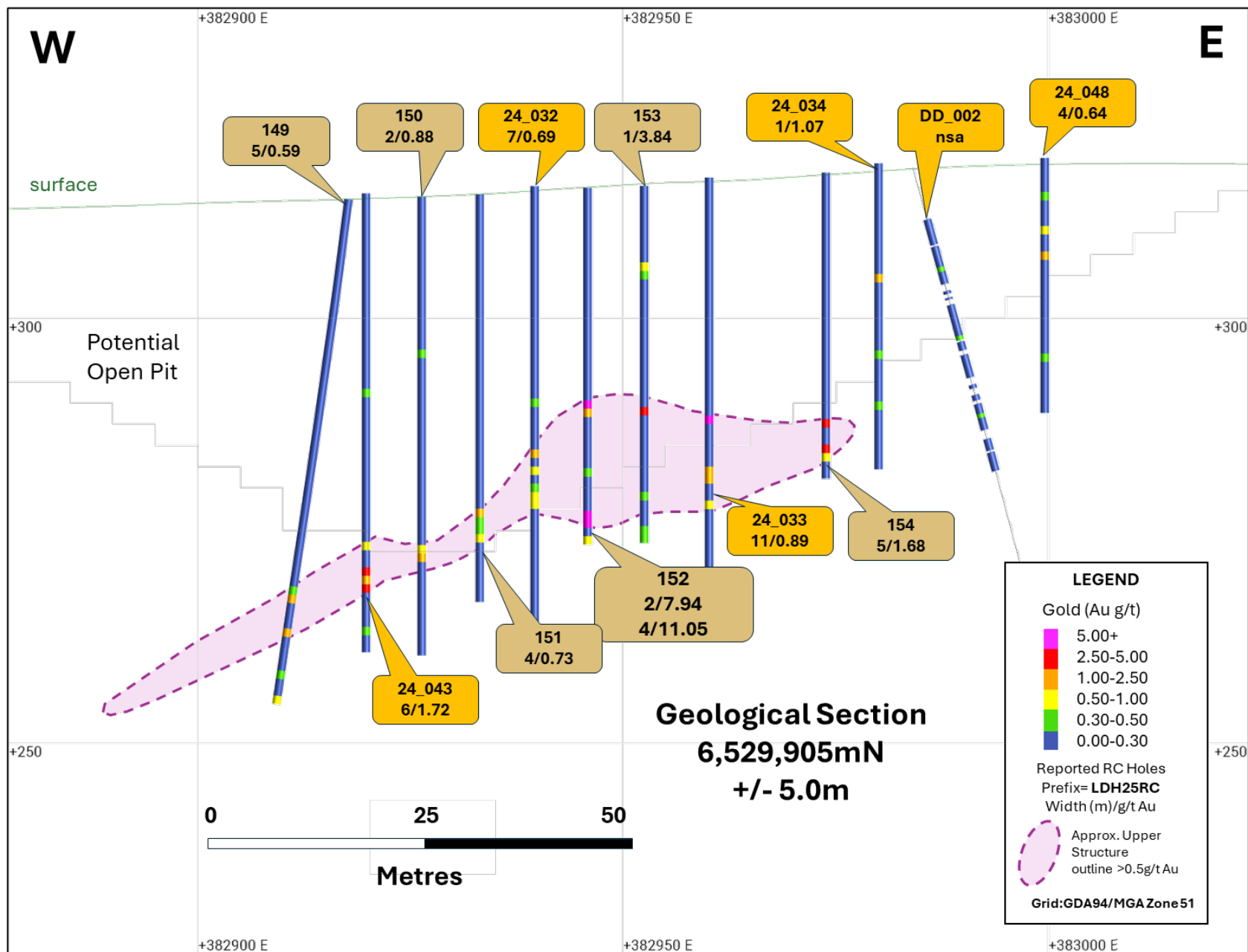
Figure 7: Section 6,529,905mN (looking north +/- 5m) illustrating the results reported today (gold call-outs) and prior reported results (orange call-outs).
