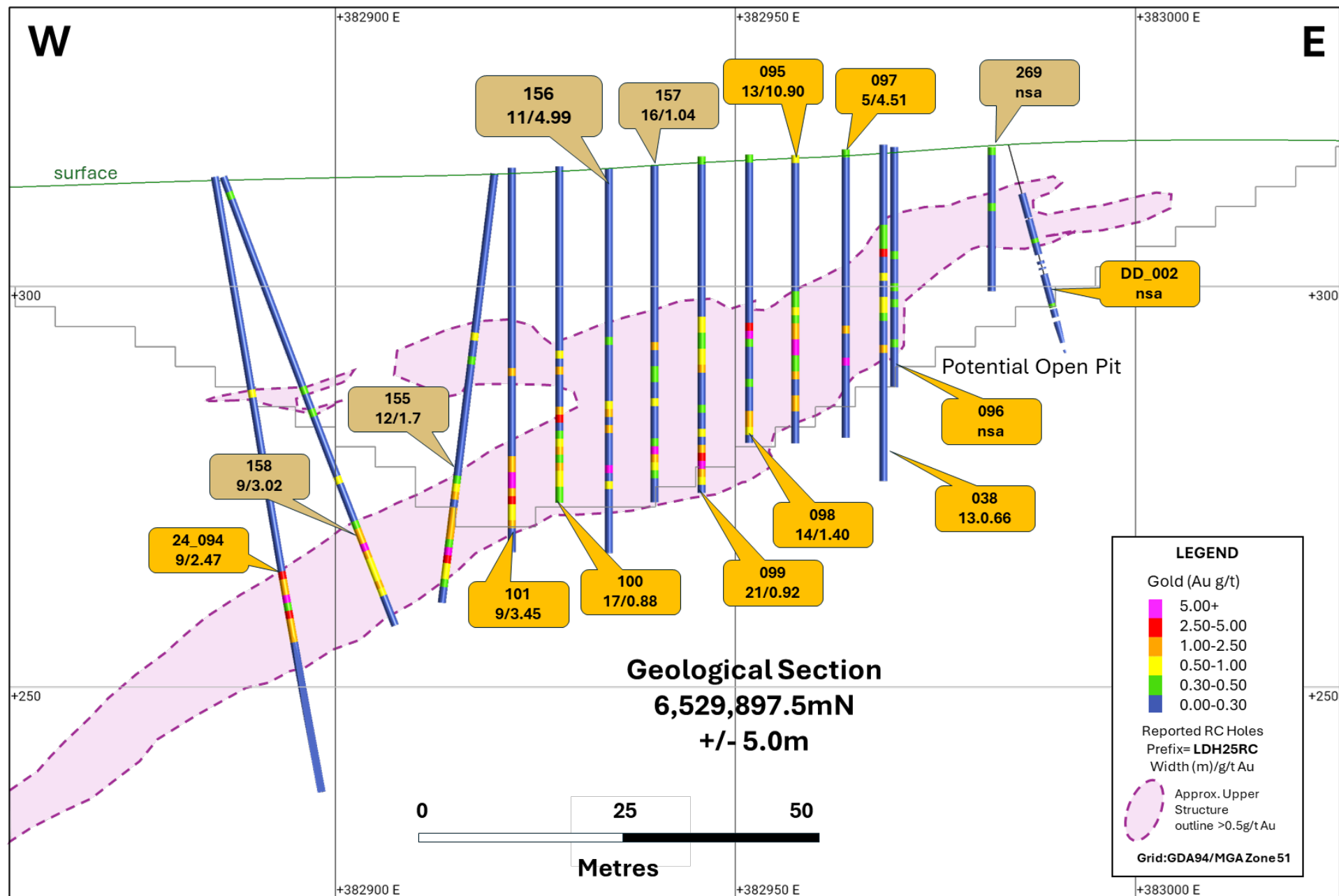
Figure 6: Section 6,529,897.5mN (looking north +/- 5m) illustrating the results reported today (gold call-outs) and prior reported results (orange call-outs).
