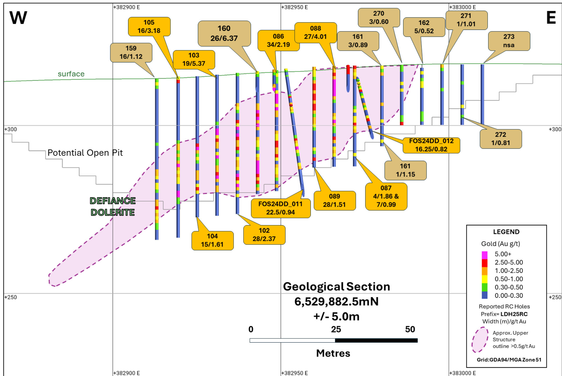
Figure 5: Section 6,529,882.5mN (looking north +/- 5m) illustrating the results reported today (gold call-outs) and prior reported results (orange call-outs).
