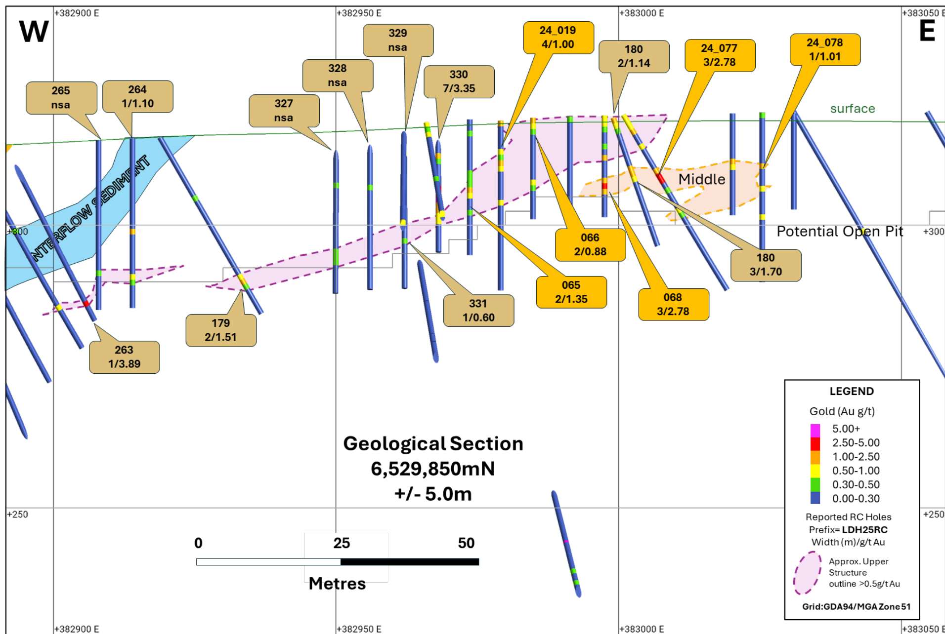
Figure 2: Section 6,529,850mN (looking north +/- 5m) illustrating the results reported today (gold call-outs) and prior reported results (orange call-outs).
