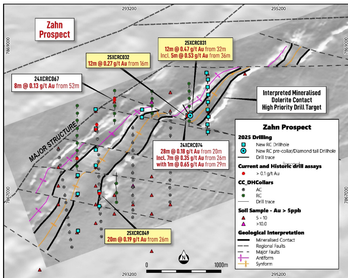
Figure 5. Plan view of the Zahn Prospect area, showing target zones, drilling with significant intercept callouts and selected soil samples above 5ppb Au. The background image is magnetics (TMI RTP 1VD) and shows an interpreted early high-mag intrusive that has been folded, providing syn- and anti-formal structures adjacent to a demagnetised structural corridor/major structure. The interpreted dolerite contacts (in solid black) represent high-priority drill targets.
