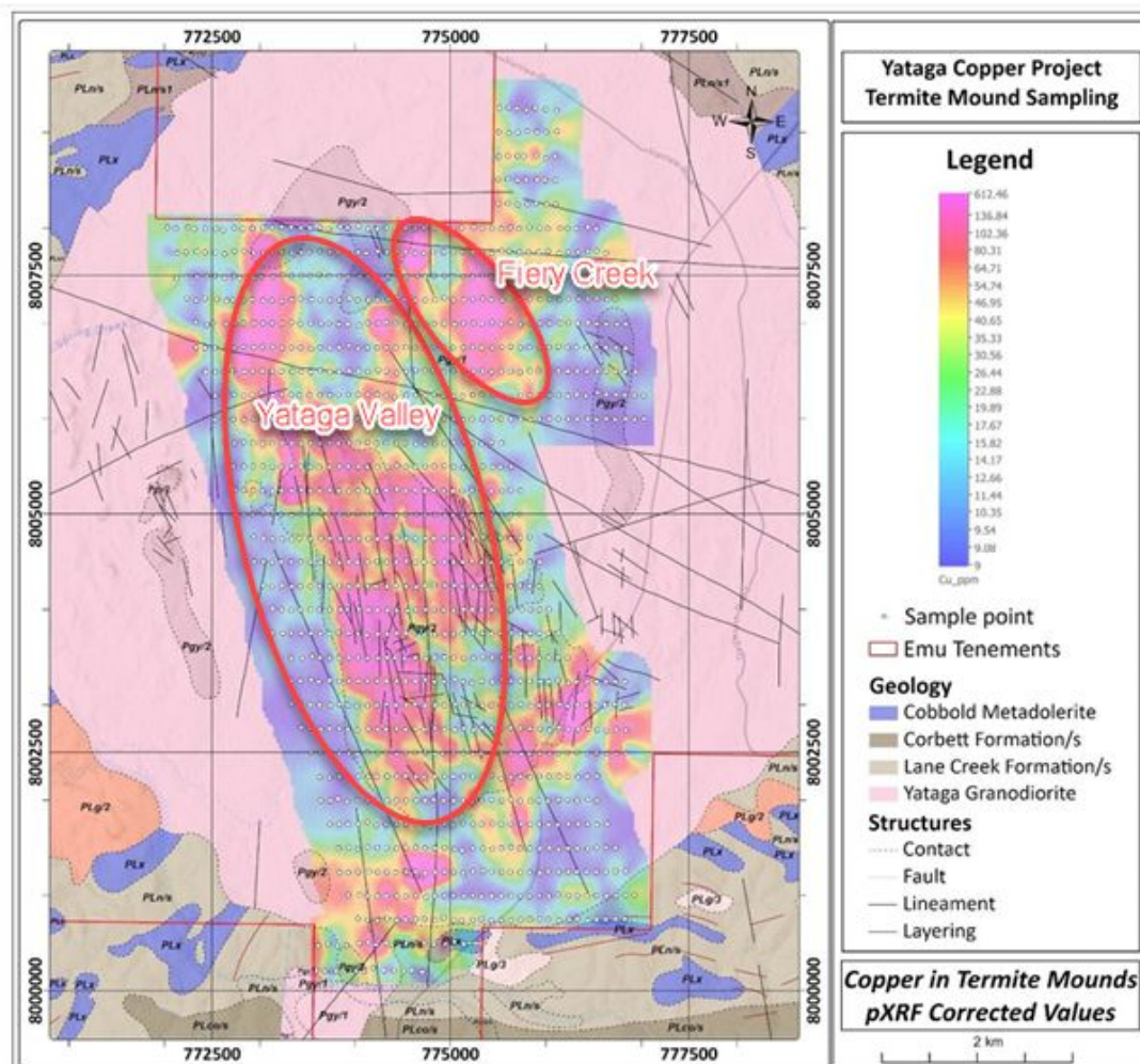
Figure 1 shows the significant copper anomalism within the Yataga Igneous Complex which includes Fiery Creek, an area of strong copper anomalism and outcropping copper mineralisation.
