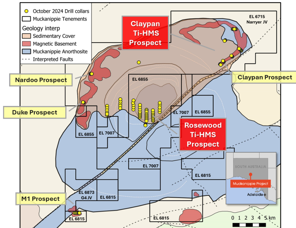
Figure 1 – Interpreted Geology Map of the Petrathern Muckanippie Project Area with prospect names and 2024 drill collars. Note Narryer JV tenement EL6715
