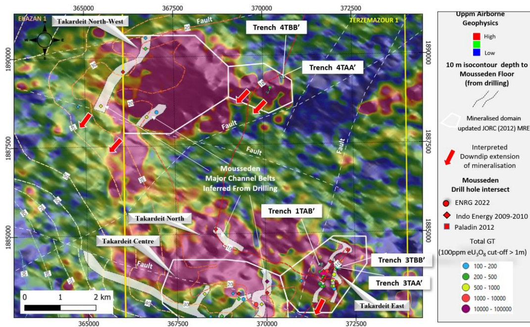
Figure 12: Inferred palaeochannel system and depth to the base of the Mousseden Formation interpreted from drilling over uranium airborne anomalies in the Takardeit northern area. 8
