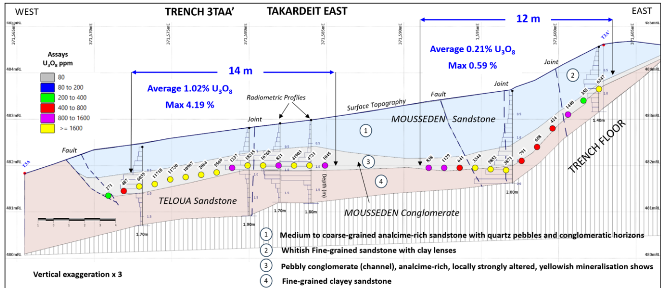
Figure 4: Trench T3AA litho-stratigraphy and uranium assay results
