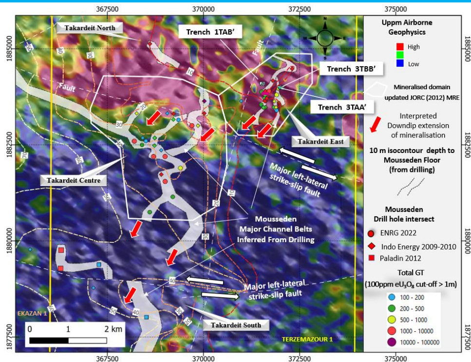
Figure 11: Inferred palaeochannel system and depth to the base of the Mousseden Formation interpreted from drilling over uranium airborne anomalies in the Takardeit region. 8
