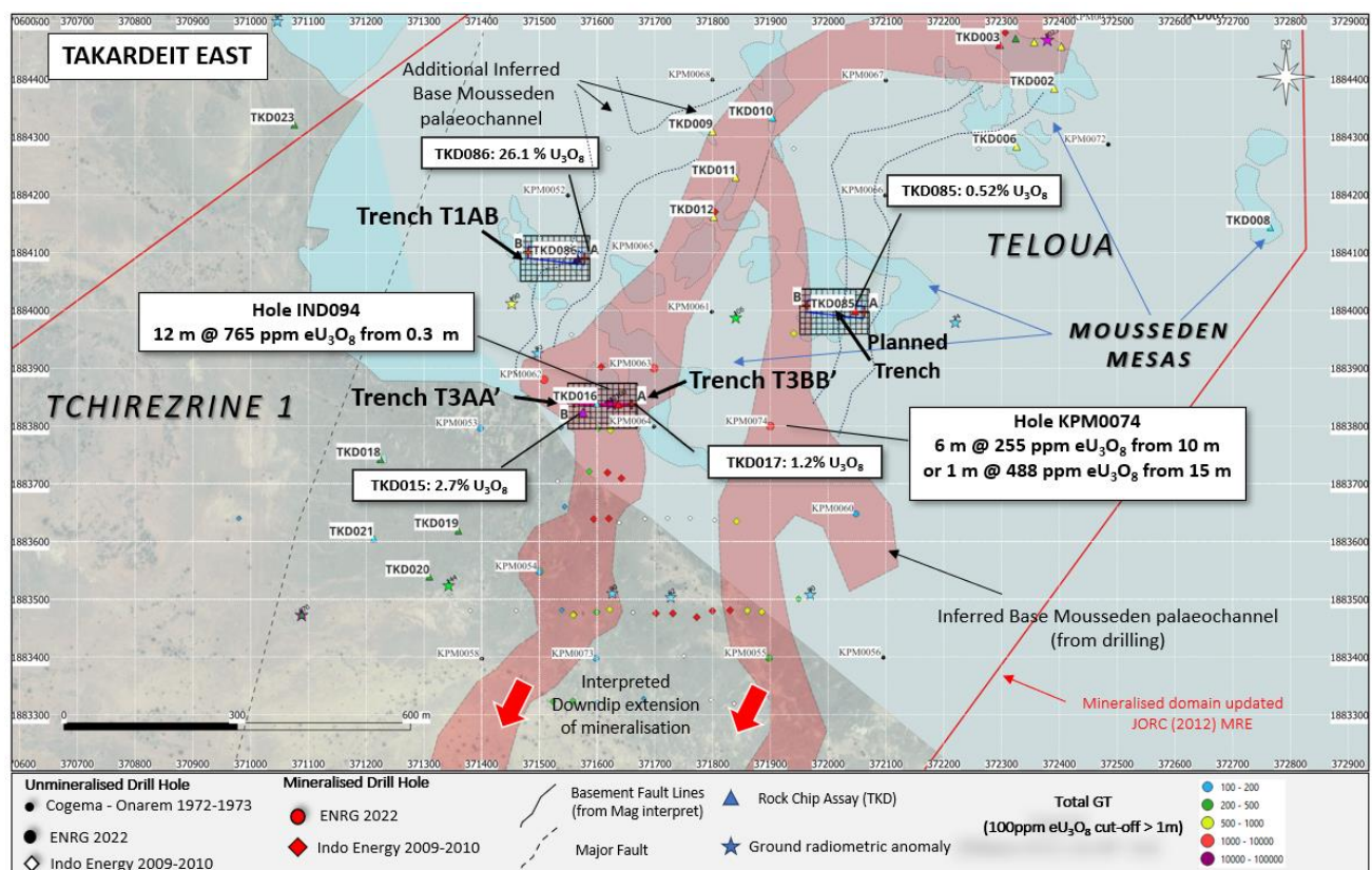
Figure 10: Interpreted Mousseden paleochannel system from drilling and trenches over Takardeit
