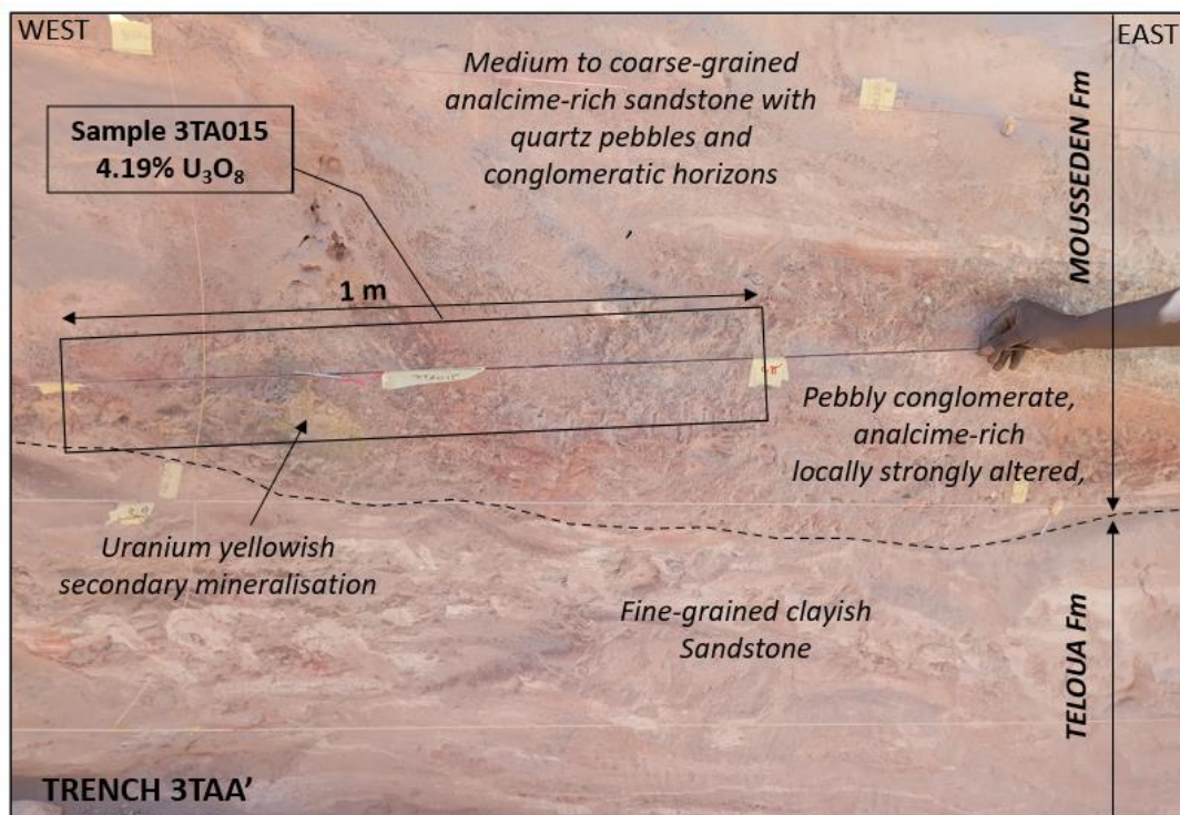
Figure 5: Lithology and uranium content in sample 3TA015, Trench T3AA'
