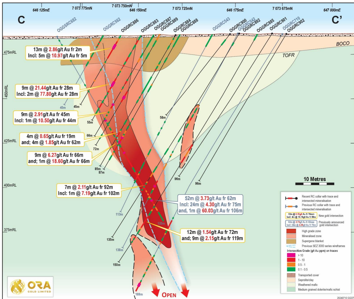
Figure 5. Cross Section C-C' at the eastern end of SEZ Mineralisation
