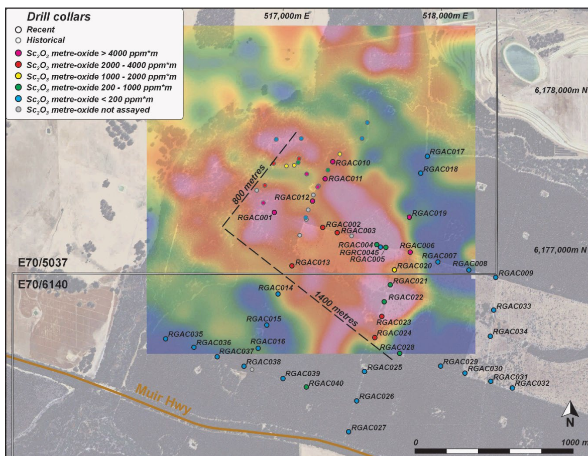
Figure 1. Map showing metre x Scandium oxide grades (ppm*m) for both recent and historical drilling at the Ivar Prospect, Rocky Gully Project, as well as recent laterite sampling ( \text{Sc}_2\text{O}_3 ppm). Note the areal extent of mineralisation. Background image is of high resolution Bouguer 1VD. (Co-ords: GDA2020 Zone 50)
