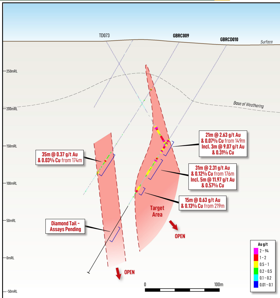
Figure 2: Gidginbung cross section illustrating the results from holes GBRC009 and GBRC010.
