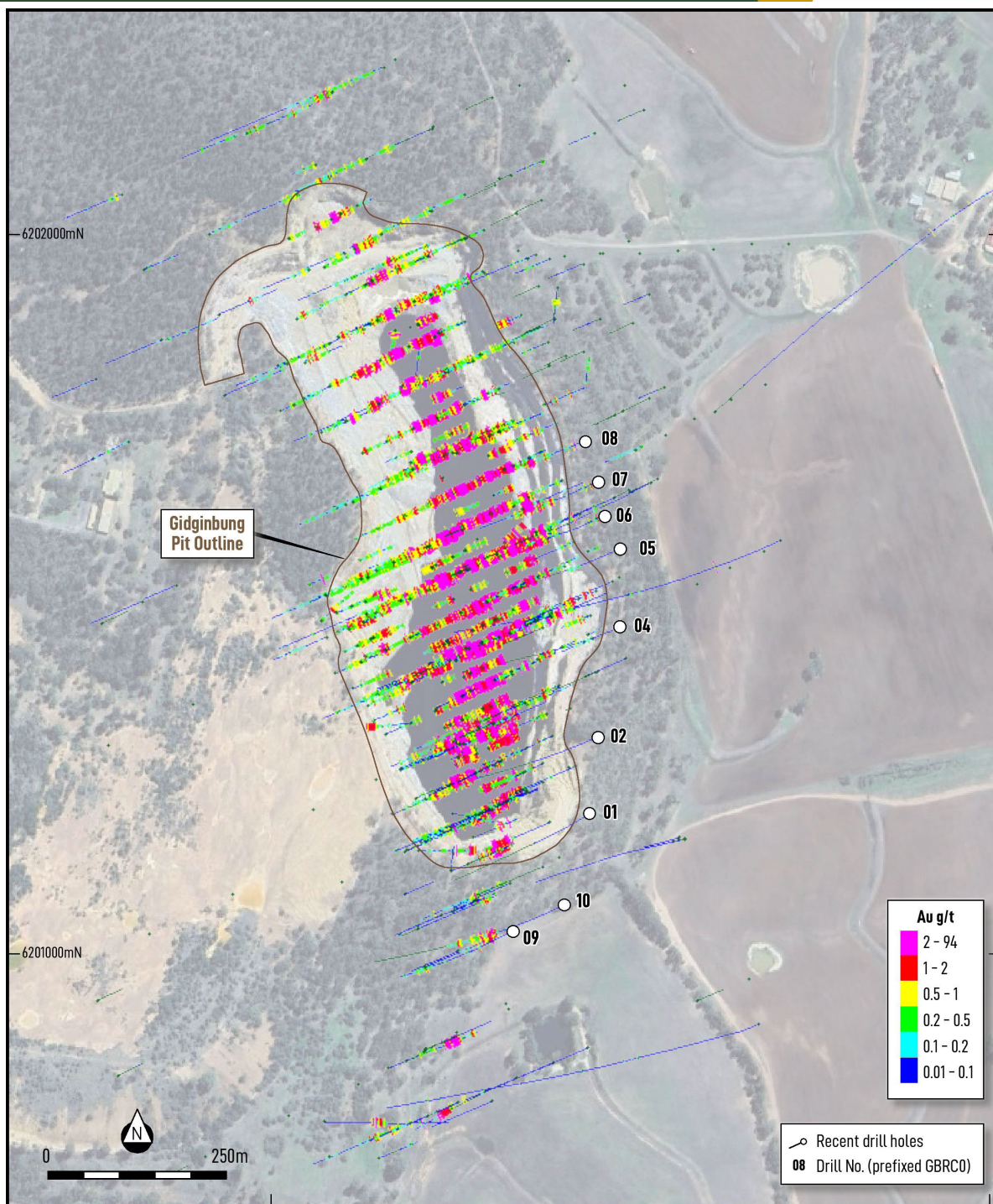
Figure 1: Gidginbung plan image illustrating the location of recent drilling results.
