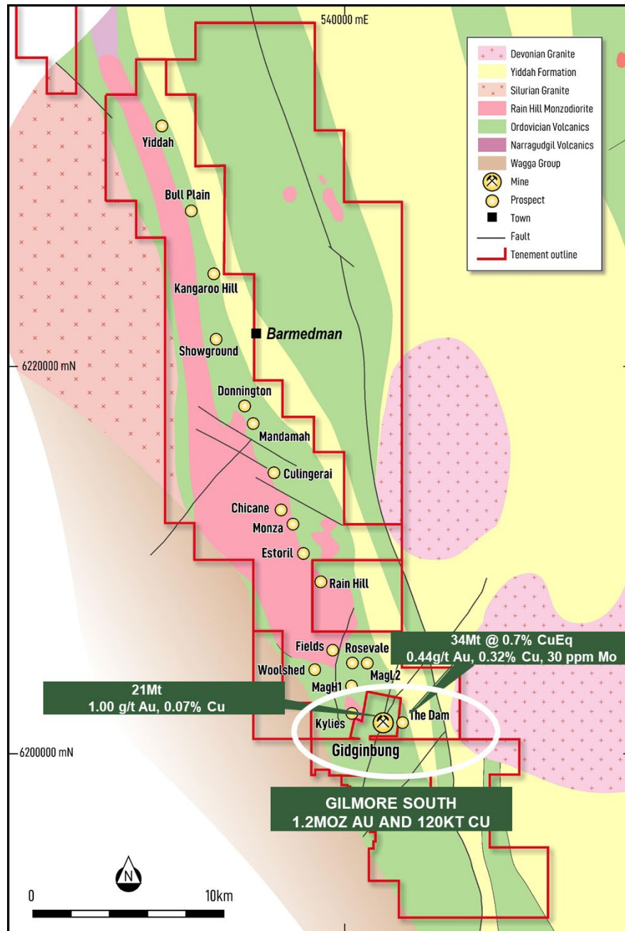
Figure 6: Plan view of the Gilmore Project including Gilmore South where the Company is currently drilling.
