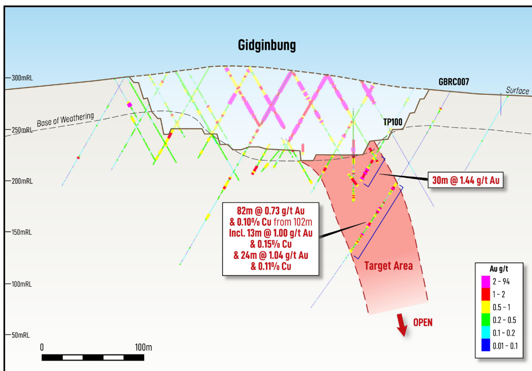
Figure 4: Gidginbung cross section illustrating the results from hole GBRC007.
