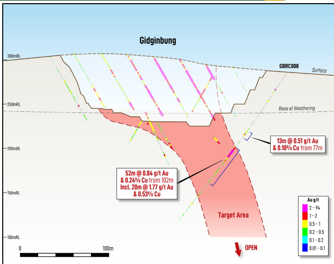
Figure 3: Gidginbung cross section illustrating the results from hole GBRC008.
