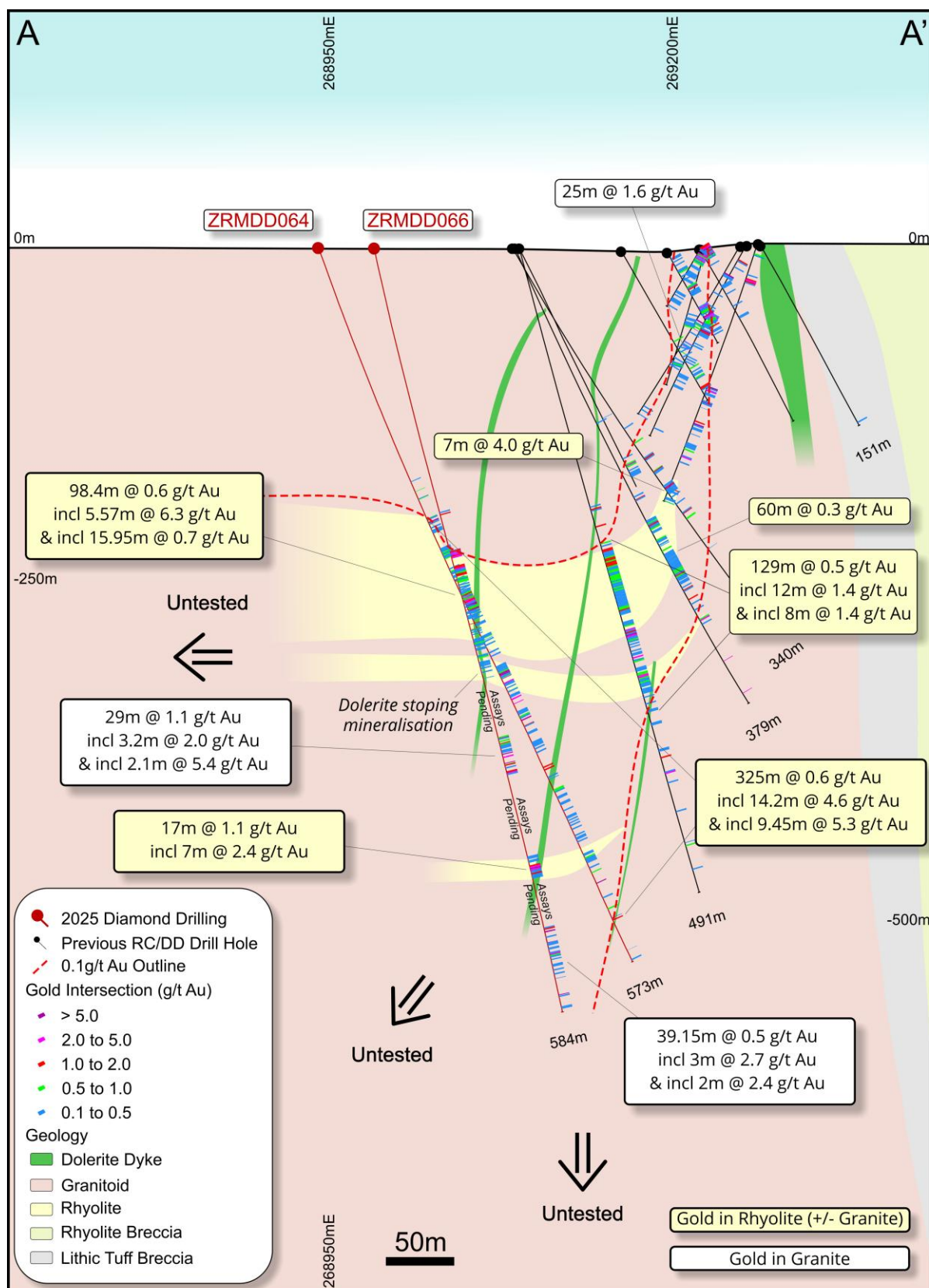
Figure 1: Cross-section (A-A') through the Red Mountain Gold Project.
