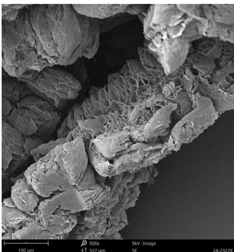
Figure 2: Scanning Electron Microscopy (SEM) of optimised expanded graphite, achieving 650cm 3 /g expansion volume.
